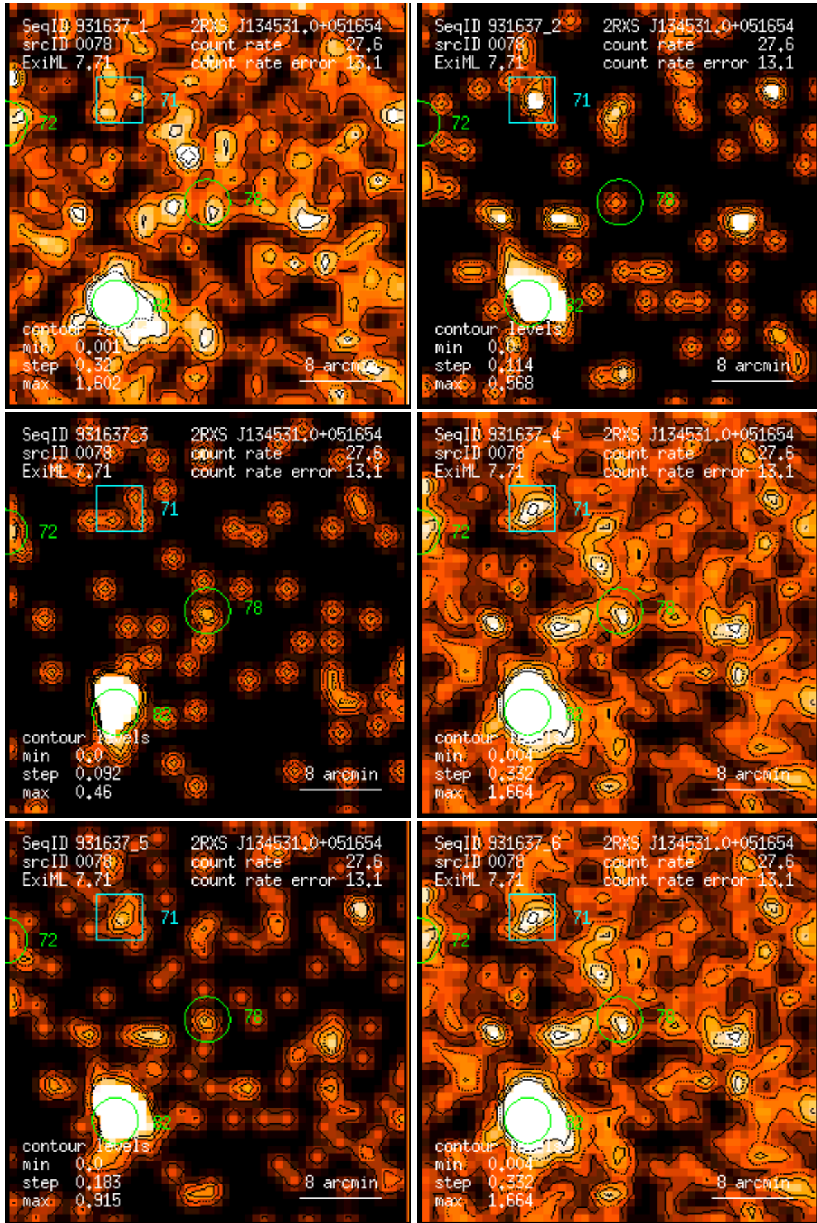
Figure 78: RASS 931637: detection 0078: band rate images, Gaussian filter: (1) PSPC channels 11 – 41, (2) 52 – 90, (3) 91 – 201, (4) 11 – 235, (5) 52 – 201, (6) 11 – 201. Broad band rates in counts/ks. Band rate contour levels in counts/ks/arcmin 2 .
