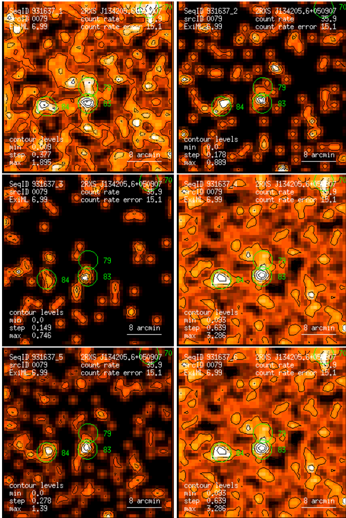
Figure 79: RASS 931637: detection 0079: band rate images, Gaussian filter: (1) PSPC channels 11 – 41, (2) 52 – 90, (3) 91 – 201, (4) 11 – 235, (5) 52 – 201, (6) 11 – 201. Broad band rates in counts/ks. Band rate contour levels in counts/ks/arcmin 2 .
