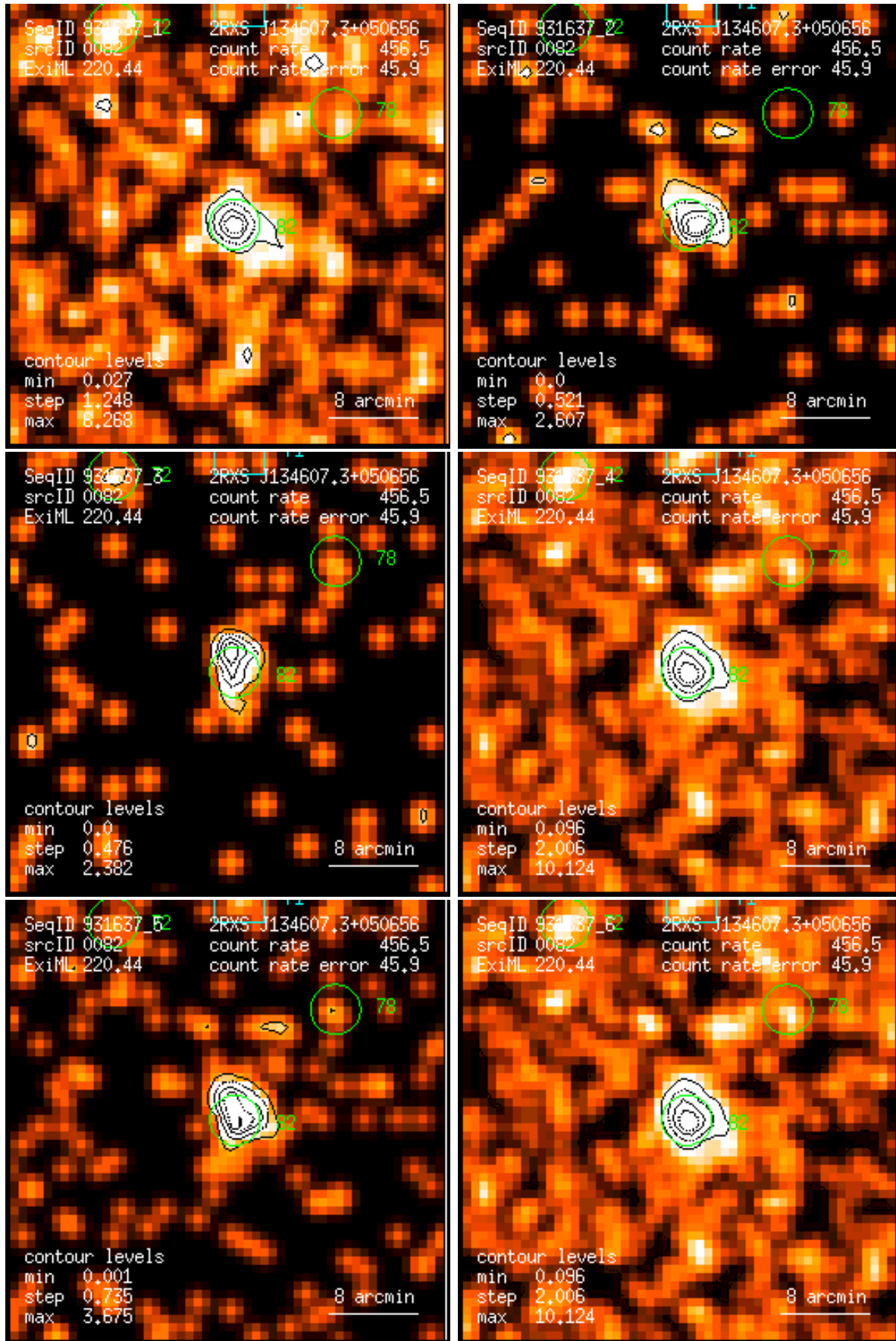
Figure 82: RASS 931637: detection 0082: band rate images, Gaussian filter: (1) PSPC channels 11 – 41, (2) 52 – 90, (3) 91 – 201, (4) 11 – 235, (5) 52 – 201, (6) 11 – 201. Broad band rates in counts/ks. Band rate contour levels in counts/ks/arcmin 2 .
