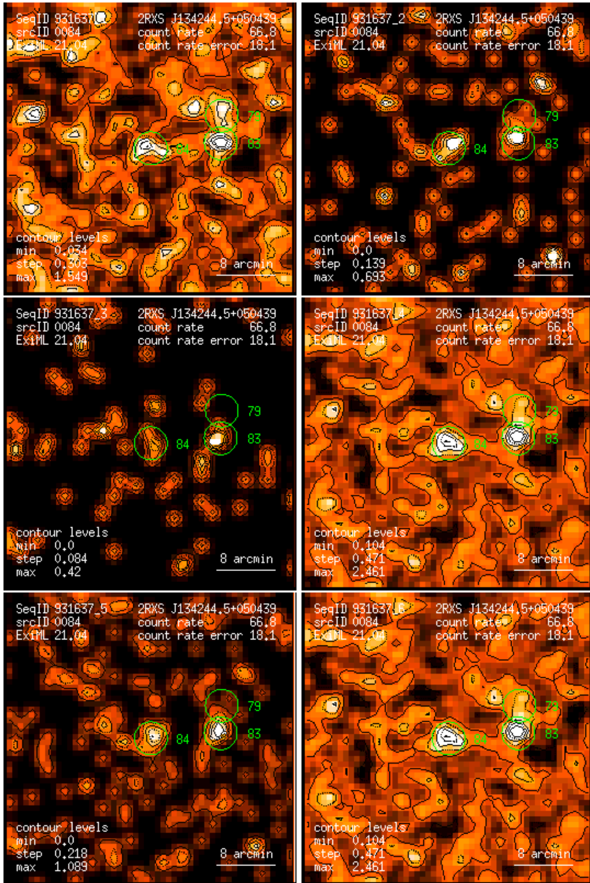
Figure 84: RASS 931637: detection 0084: band rate images, Gaussian filter: (1) PSPC channels 11 – 41, (2) 52 – 90, (3) 91 – 201, (4) 11 – 235, (5) 52 – 201, (6) 11 – 201. Broad band rates in counts/ks. Band rate contour levels in counts/ks/arcmin 2 .
