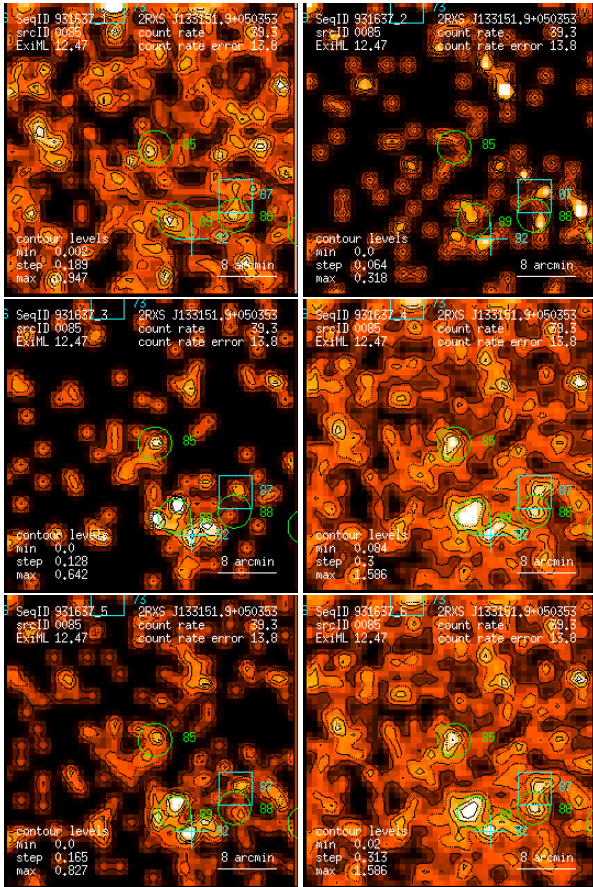
Figure 85: RASS 931637: detection 0085: band rate images, Gaussian filter: (1) PSPC channels 11 – 41, (2) 52 – 90, (3) 91 – 201, (4) 11 – 235, (5) 52 – 201, (6) 11 – 201. Broad band rates in counts/ks. Band rate contour levels in counts/ks/arcmin 2 .
