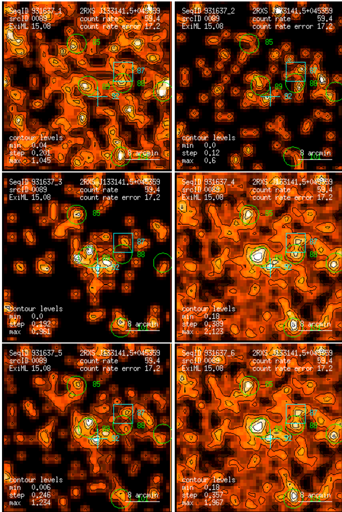
Figure 89: RASS 931637: detection 0089: band rate images, Gaussian filter: (1) PSPC channels 11 – 41, (2) 52 – 90, (3) 91 – 201, (4) 11 – 235, (5) 52 – 201, (6) 11 – 201. Broad band rates in counts/ks. Band rate contour levels in counts/ks/arcmin 2 .
