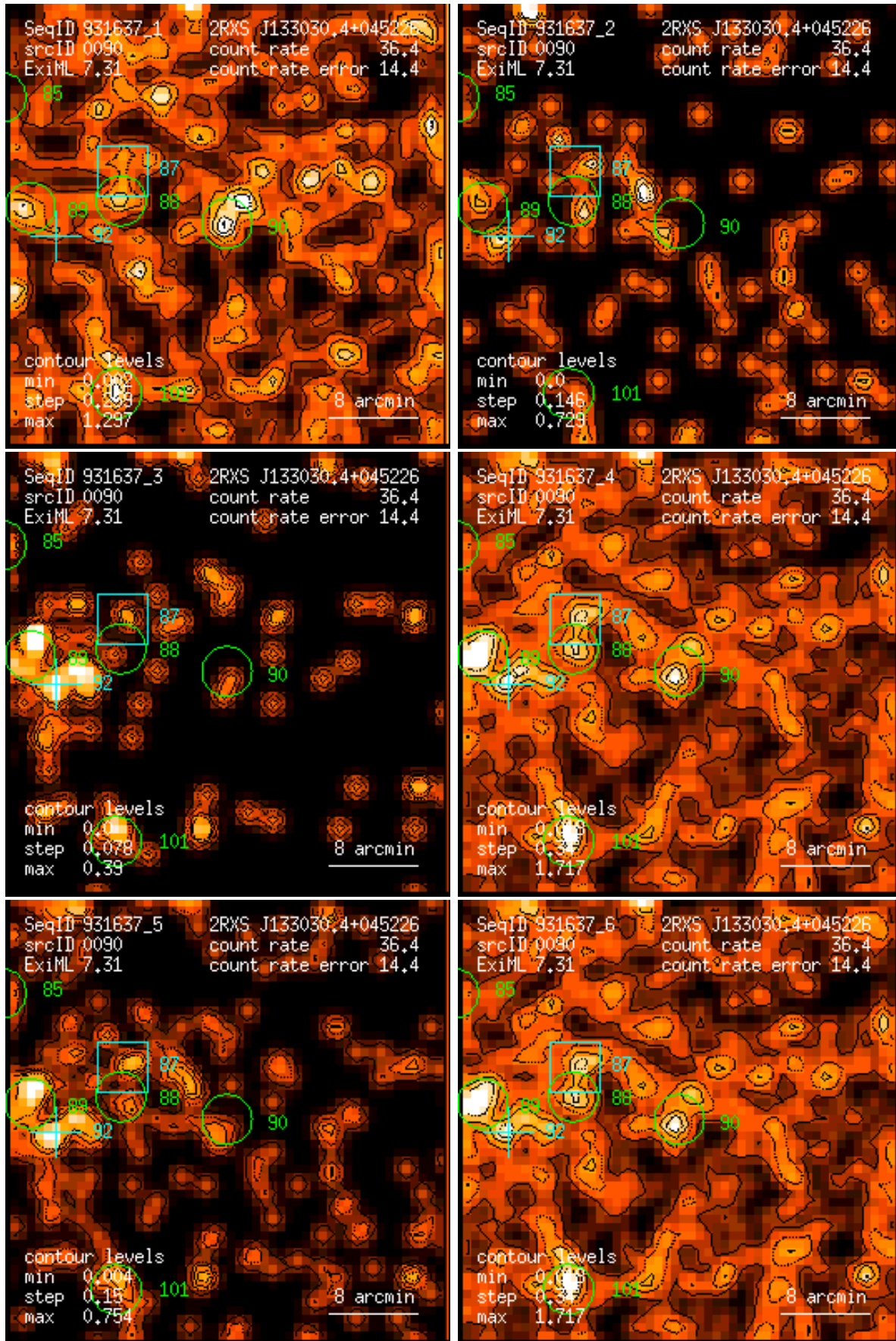
Figure 90: RASS 931637: detection 0090: band rate images, Gaussian filter: (1) PSPC channels 11 – 41, (2) 52 – 90, (3) 91 – 201, (4) 11 – 235, (5) 52 – 201, (6) 11 – 201. Broad band rates in counts/ks. Band rate contour levels in counts/ks/arcmin 2 .
