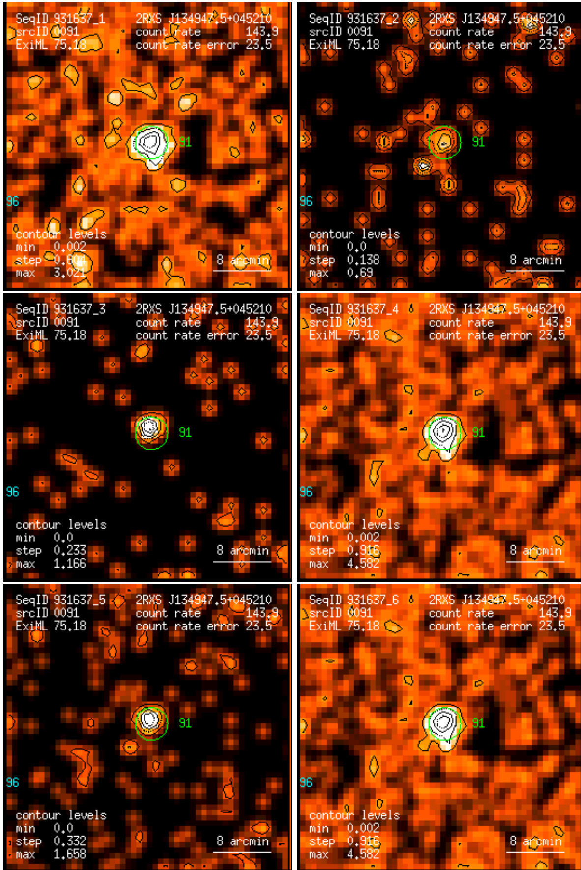
Figure 91: RASS 931637: detection 0091: band rate images, Gaussian filter: (1) PSPC channels 11 – 41, (2) 52 – 90, (3) 91 – 201, (4) 11 – 235, (5) 52 – 201, (6) 11 – 201. Broad band rates in counts/ks. Band rate contour levels in counts/ks/arcmin 2 .
