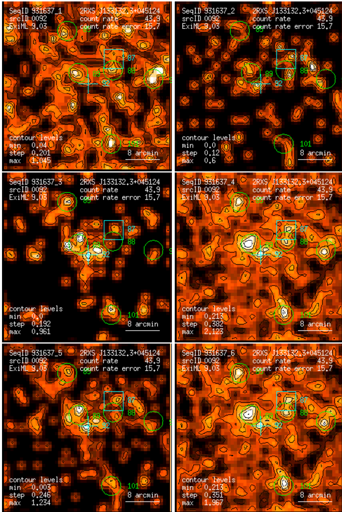
Figure 92: RASS 931637: detection 0092: band rate images, Gaussian filter: (1) PSPC channels 11 – 41, (2) 52 – 90, (3) 91 – 201, (4) 11 – 235, (5) 52 – 201, (6) 11 – 201. Broad band rates in counts/ks. Band rate contour levels in counts/ks/arcmin 2 .
