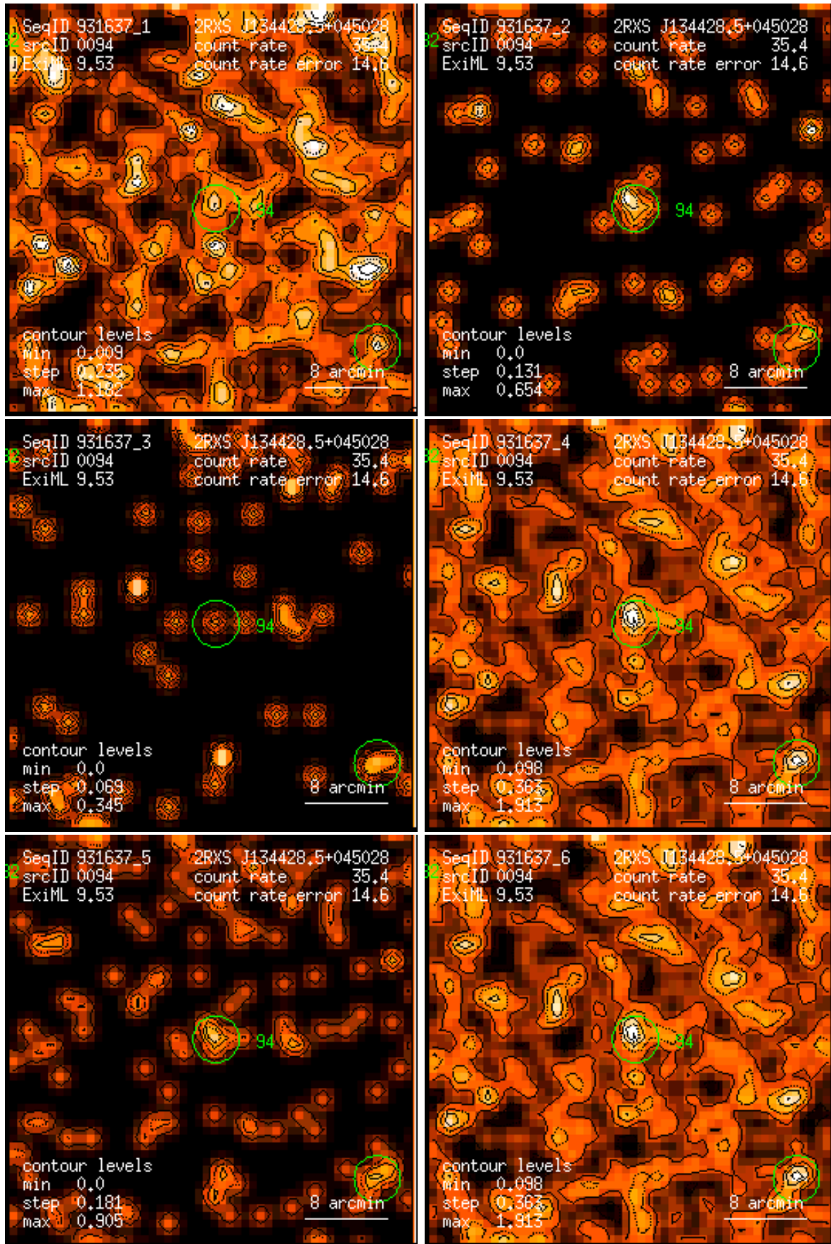
Figure 94: RASS 931637: detection 0094: band rate images, Gaussian filter: (1) PSPC channels 11 – 41, (2) 52 – 90, (3) 91 – 201, (4) 11 – 235, (5) 52 – 201, (6) 11 – 201. Broad band rates in counts/ks. Band rate contour levels in counts/ks/arcmin 2 .
