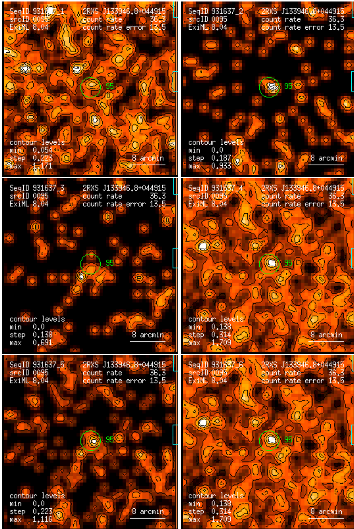
Figure 95: RASS 931637: detection 0095: band rate images, Gaussian filter: (1) PSPC channels 11 – 41, (2) 52 – 90, (3) 91 – 201, (4) 11 – 235, (5) 52 – 201, (6) 11 – 201. Broad band rates in counts/ks. Band rate contour levels in counts/ks/arcmin 2 .
