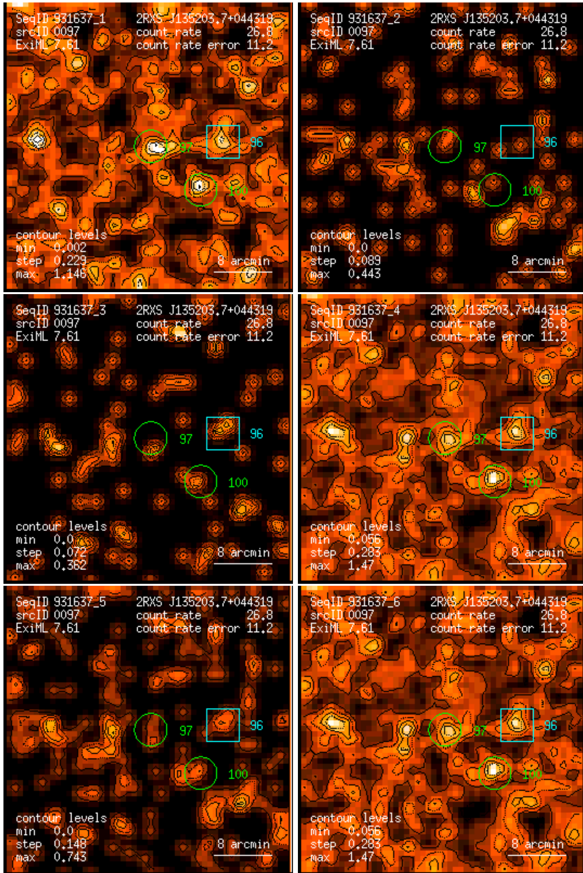
Figure 97: RASS 931637: detection 0097: band rate images, Gaussian filter: (1) PSPC channels 11 – 41, (2) 52 – 90, (3) 91 – 201, (4) 11 – 235, (5) 52 – 201, (6) 11 – 201. Broad band rates in counts/ks. Band rate contour levels in counts/ks/arcmin 2 .
