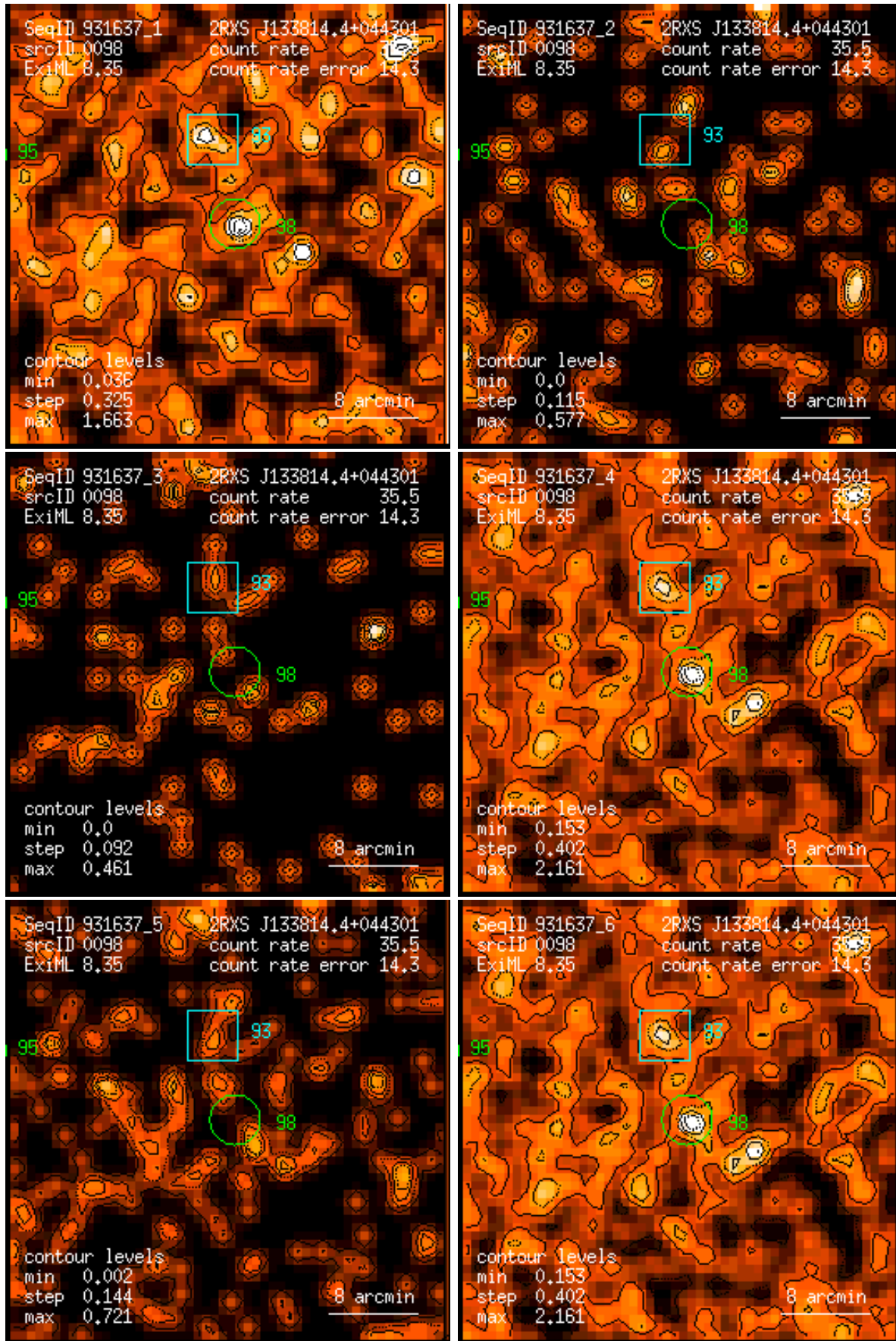
Figure 98: RASS 931637: detection 0098: band rate images, Gaussian filter: (1) PSPC channels 11 – 41, (2) 52 – 90, (3) 91 – 201, (4) 11 – 235, (5) 52 – 201, (6) 11 – 201. Broad band rates in counts/ks. Band rate contour levels in counts/ks/arcmin 2 .
