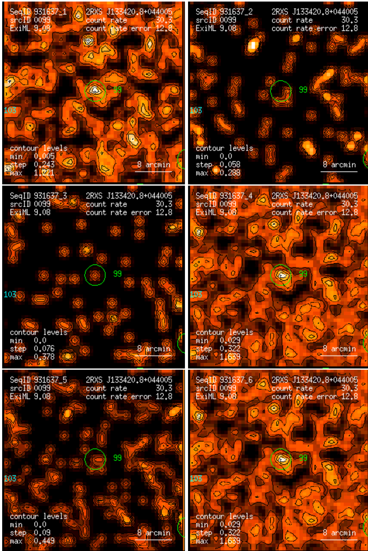
Figure 99: RASS 931637: detection 0099: band rate images, Gaussian filter: (1) PSPC channels 11 – 41, (2) 52 – 90, (3) 91 – 201, (4) 11 – 235, (5) 52 – 201, (6) 11 – 201. Broad band rates in counts/ks. Band rate contour levels in counts/ks/arcmin 2 .
