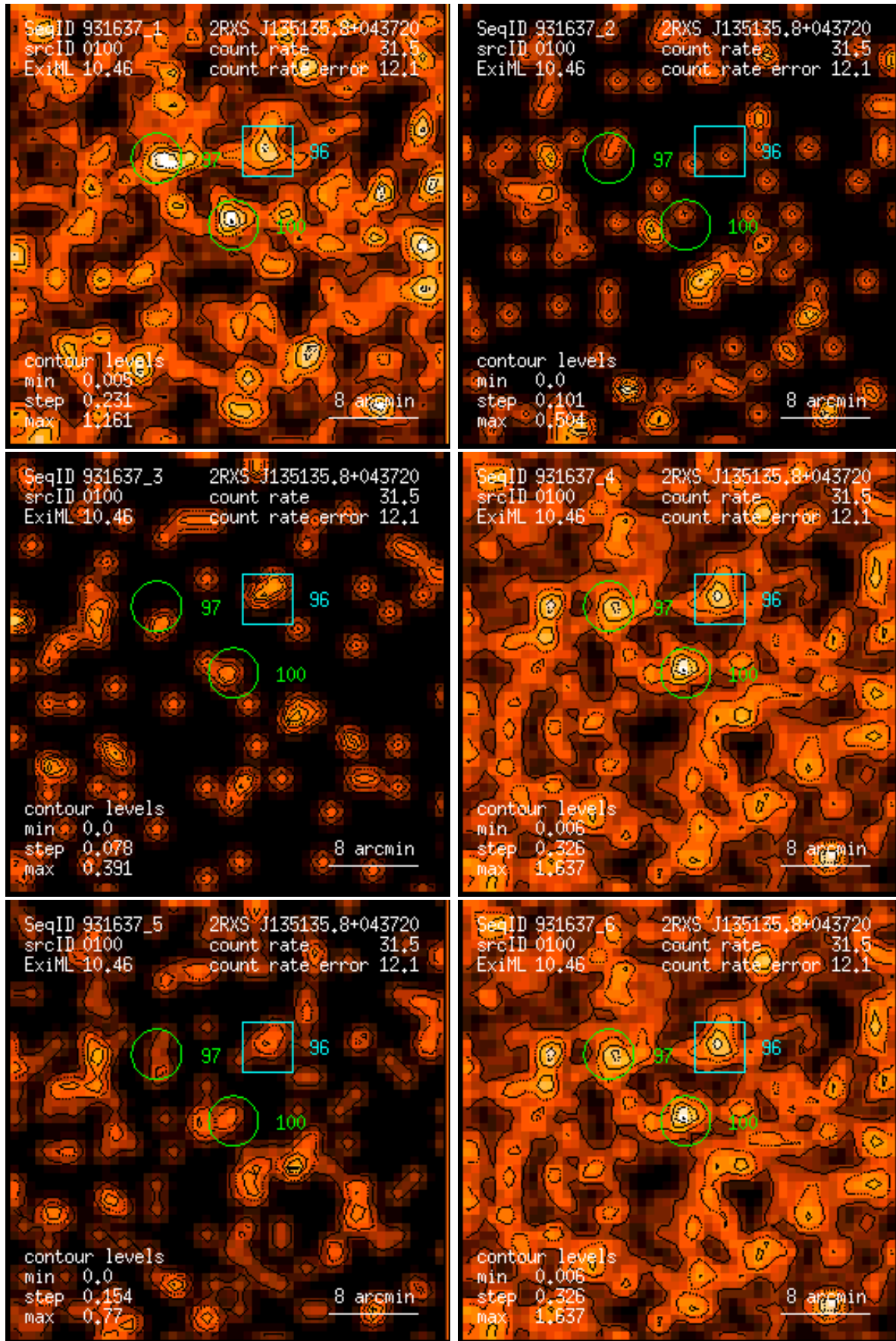
Figure 100: RASS 931637: detection 0100: band rate images, Gaussian filter: (1) PSPC channels 11 – 41, (2) 52 – 90, (3) 91 – 201, (4) 11 – 235, (5) 52 – 201, (6) 11 – 201. Broad band rates in counts/ks. Band rate contour levels in counts/ks/arcmin 2 .
