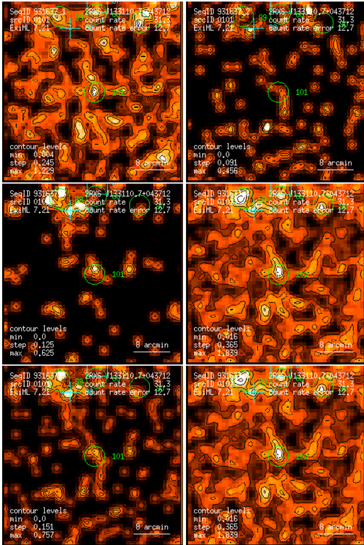
Figure 101: RASS 931637: detection 0101: band rate images, Gaussian filter: (1) PSPC channels 11 – 41, (2) 52 – 90, (3) 91 – 201, (4) 11 – 235, (5) 52 – 201, (6) 11 – 201. Broad band rates in counts/ks. Band rate contour levels in counts/ks/arcmin 2 .
