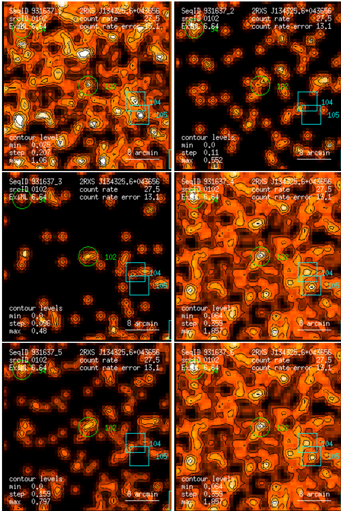
Figure 102: RASS 931637: detection 0102: band rate images, Gaussian filter: (1) PSPC channels 11 – 41, (2) 52 – 90, (3) 91 – 201, (4) 11 – 235, (5) 52 – 201, (6) 11 – 201. Broad band rates in counts/ks. Band rate contour levels in counts/ks/arcmin 2 .
