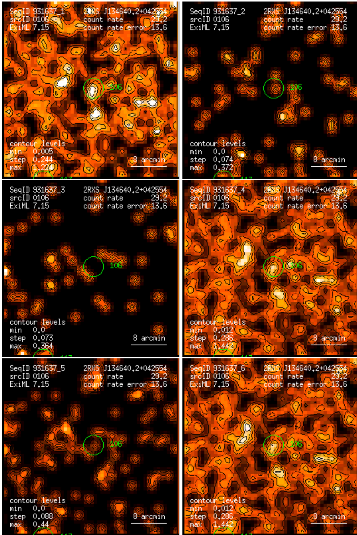
Figure 106: RASS 931637: detection 0106: band rate images, Gaussian filter: (1) PSPC channels 11 – 41, (2) 52 – 90, (3) 91 – 201, (4) 11 – 235, (5) 52 – 201, (6) 11 – 201. Broad band rates in counts/ks. Band rate contour levels in counts/ks/arcmin 2 .
