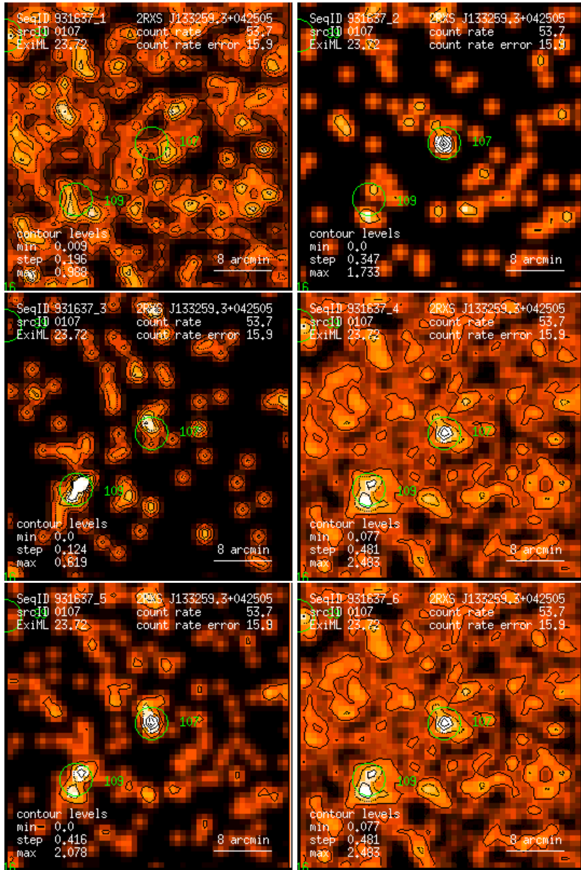
Figure 107: RASS 931637: detection 0107: band rate images, Gaussian filter: (1) PSPC channels 11 – 41, (2) 52 – 90, (3) 91 – 201, (4) 11 – 235, (5) 52 – 201, (6) 11 – 201. Broad band rates in counts/ks. Band rate contour levels in counts/ks/arcmin 2 .
