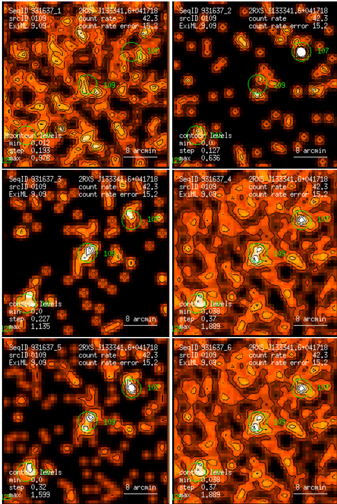
Figure 109: RASS 931637: detection 0109: band rate images, Gaussian filter: (1) PSPC channels 11 – 41, (2) 52 – 90, (3) 91 – 201, (4) 11 – 235, (5) 52 – 201, (6) 11 – 201. Broad band rates in counts/ks. Band rate contour levels in counts/ks/arcmin 2 .
