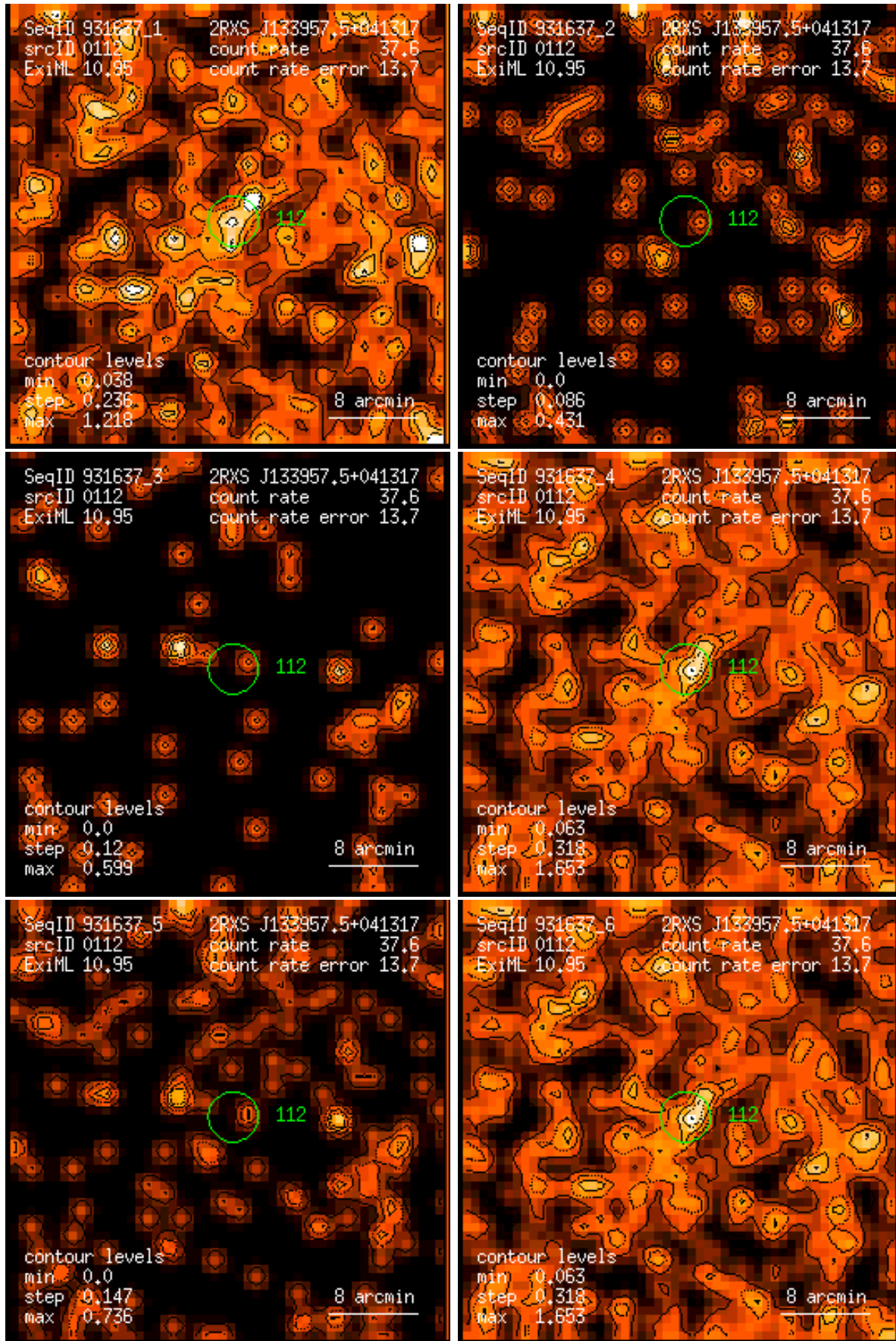
Figure 112: RASS 931637: detection 0112: band rate images, Gaussian filter: (1) PSPC channels 11 – 41, (2) 52 – 90, (3) 91 – 201, (4) 11 – 235, (5) 52 – 201, (6) 11 – 201. Broad band rates in counts/ks. Band rate contour levels in counts/ks/arcmin 2 .
