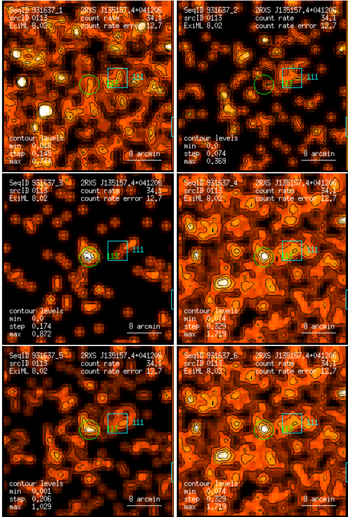
Figure 113: RASS 931637: detection 0113: band rate images, Gaussian filter: (1) PSPC channels 11 – 41, (2) 52 – 90, (3) 91 – 201, (4) 11 – 235, (5) 52 – 201, (6) 11 – 201. Broad band rates in counts/ks. Band rate contour levels in counts/ks/arcmin 2 .
