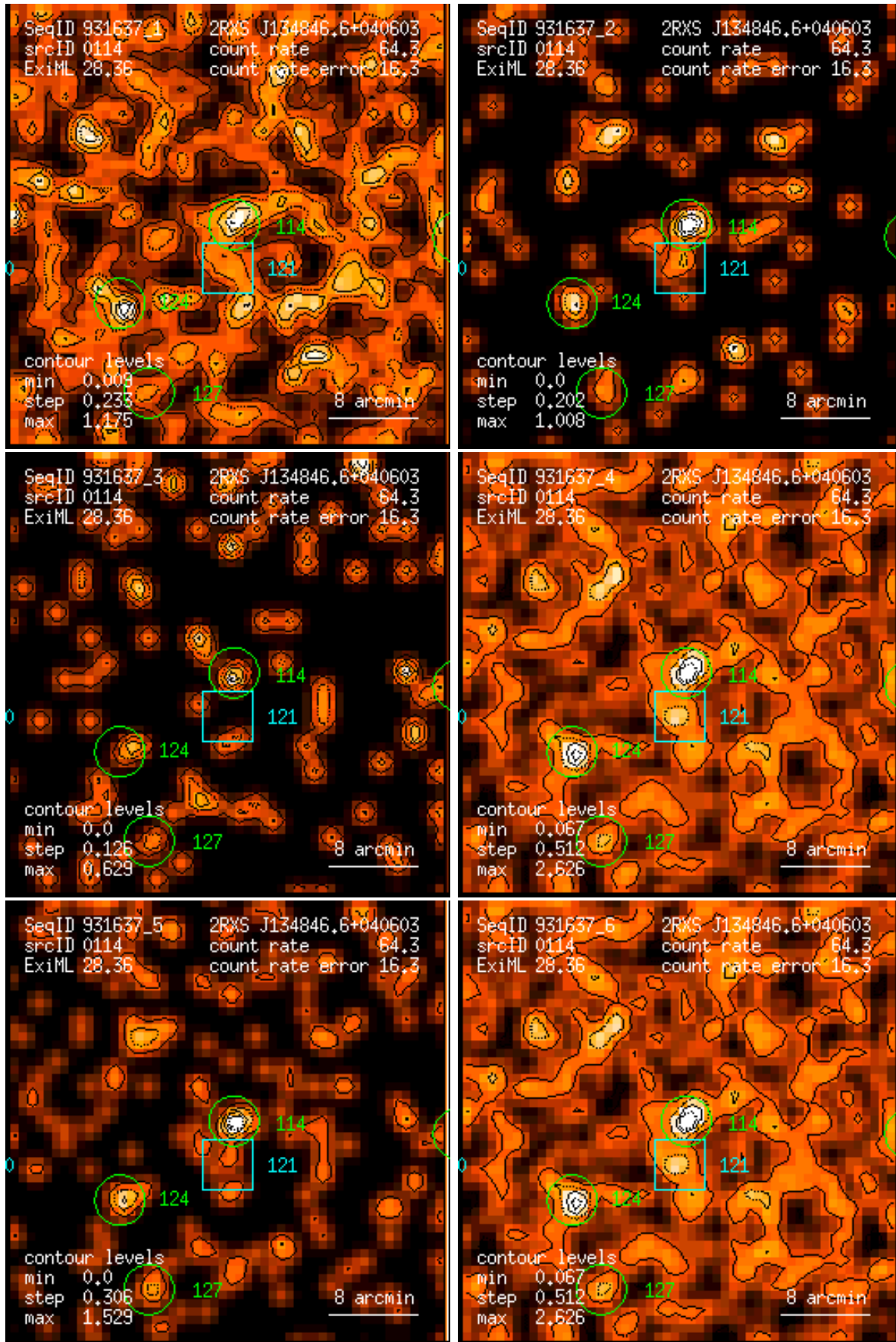
Figure 114: RASS 931637: detection 0114: band rate images, Gaussian filter: (1) PSPC channels 11 – 41, (2) 52 – 90, (3) 91 – 201, (4) 11 – 235, (5) 52 – 201, (6) 11 – 201. Broad band rates in counts/ks. Band rate contour levels in counts/ks/arcmin 2 .
