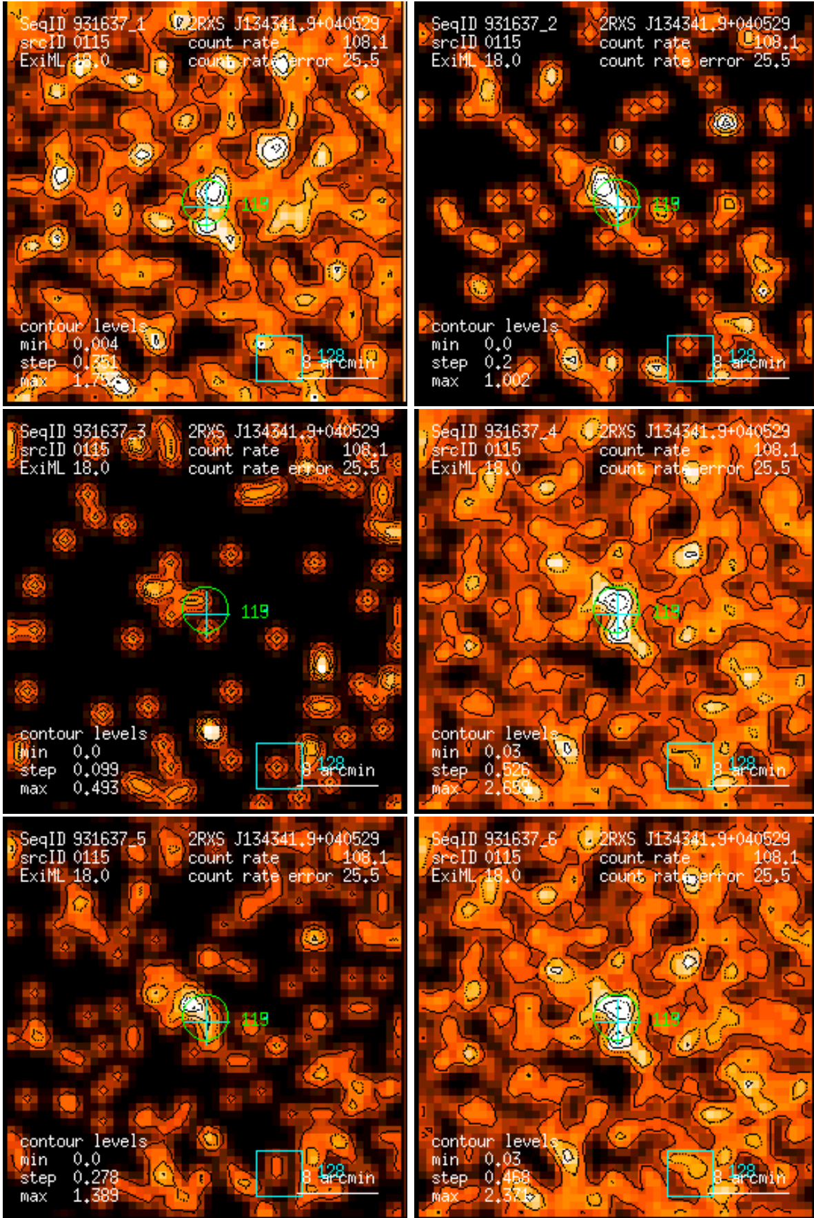
Figure 115: RASS 931637: detection 0115: band rate images, Gaussian filter: (1) PSPC channels 11 – 41, (2) 52 – 90, (3) 91 – 201, (4) 11 – 235, (5) 52 – 201, (6) 11 – 201. Broad band rates in counts/ks. Band rate contour levels in counts/ks/arcmin 2 .
