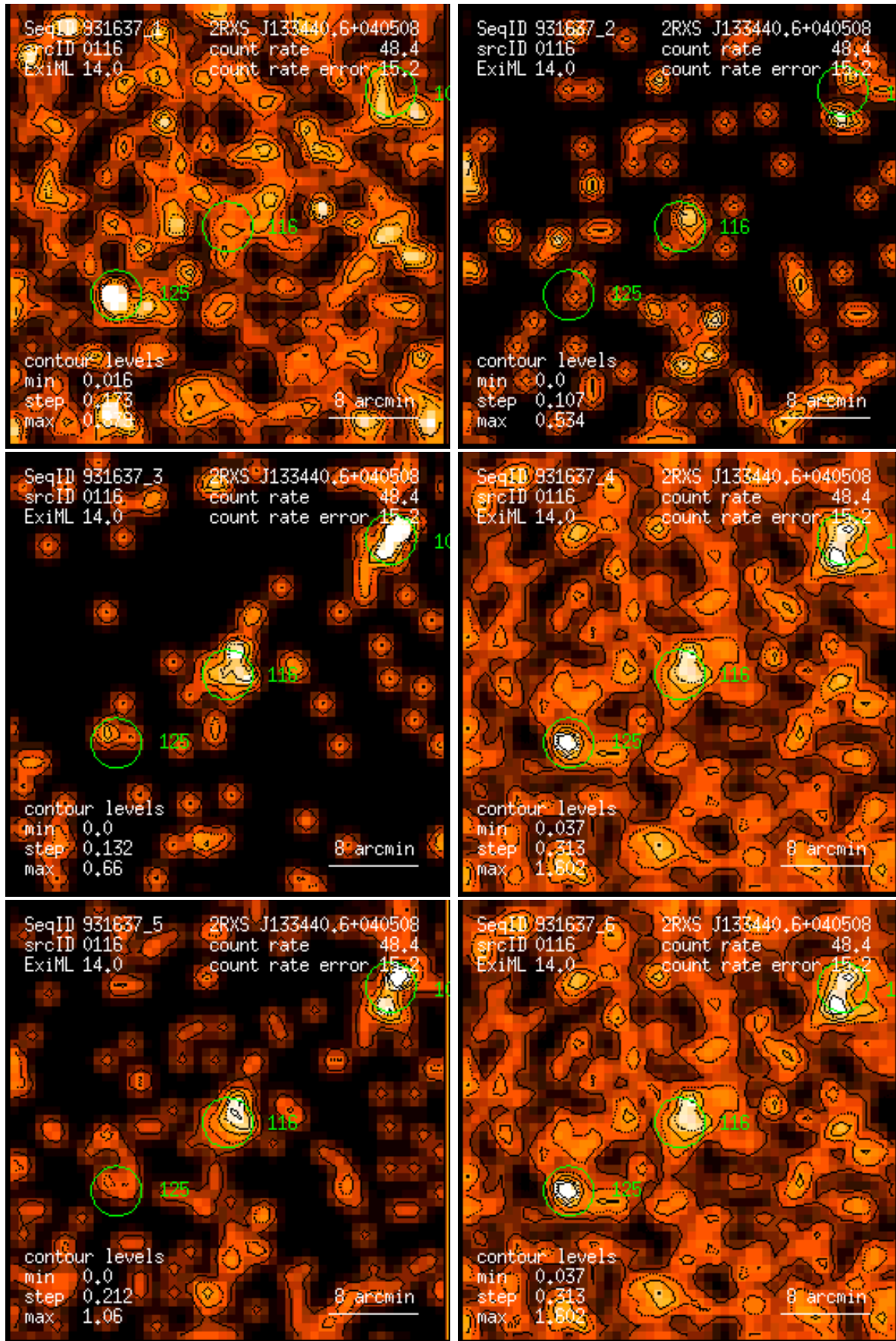
Figure 116: RASS 931637: detection 0116: band rate images, Gaussian filter: (1) PSPC channels 11 – 41, (2) 52 – 90, (3) 91 – 201, (4) 11 – 235, (5) 52 – 201, (6) 11 – 201. Broad band rates in counts/ks. Band rate contour levels in counts/ks/arcmin 2 .
