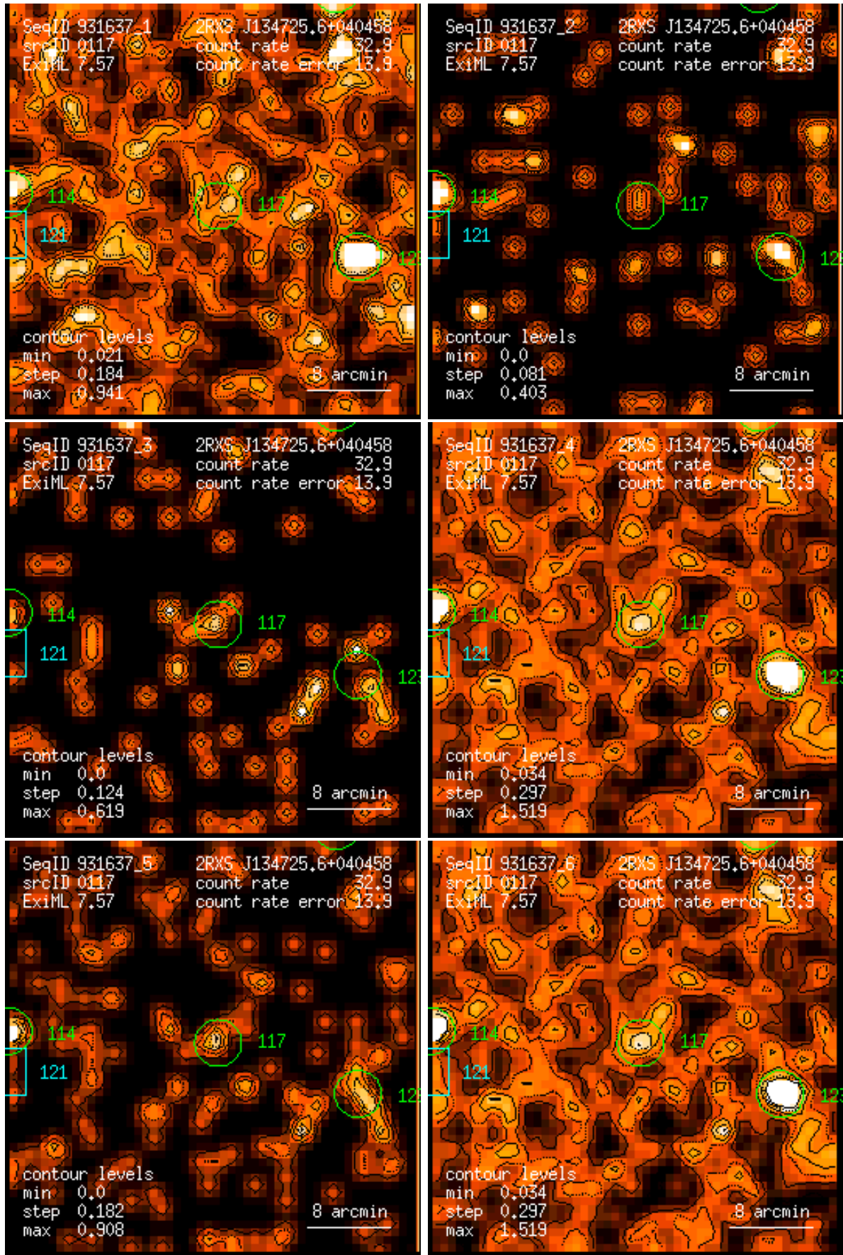
Figure 117: RASS 931637: detection 0117: band rate images, Gaussian filter: (1) PSPC channels 11 – 41, (2) 52 – 90, (3) 91 – 201, (4) 11 – 235, (5) 52 – 201, (6) 11 – 201. Broad band rates in counts/ks. Band rate contour levels in counts/ks/arcmin 2 .
