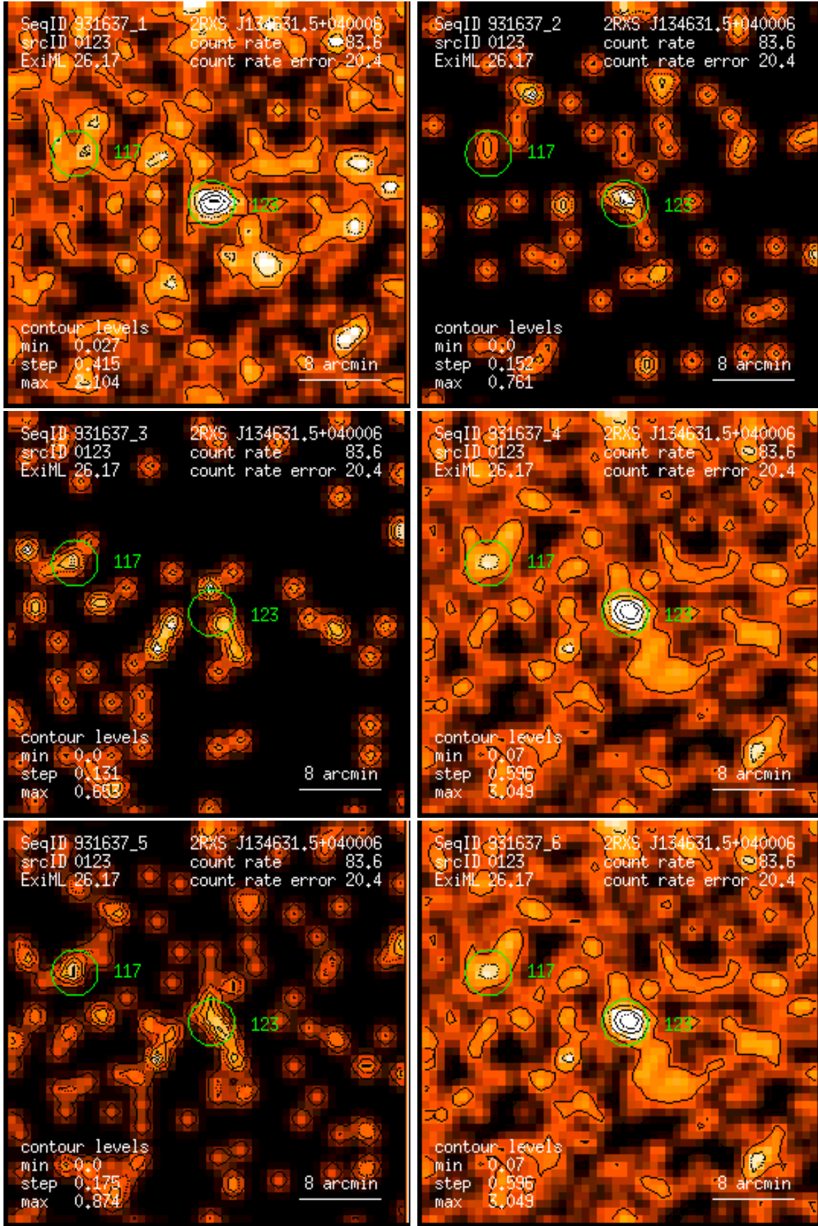
Figure 123: RASS 931637: detection 0123: band rate images, Gaussian filter: (1) PSPC channels 11 – 41, (2) 52 – 90, (3) 91 – 201, (4) 11 – 235, (5) 52 – 201, (6) 11 – 201. Broad band rates in counts/ks. Band rate contour levels in counts/ks/arcmin 2 .
