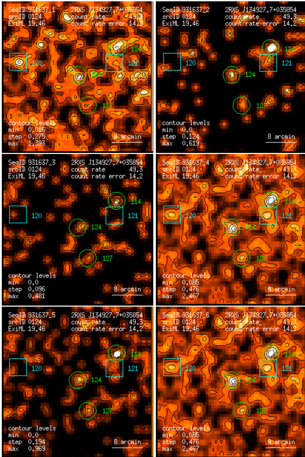
Figure 124: RASS 931637: detection 0124: band rate images, Gaussian filter: (1) PSPC channels 11 – 41, (2) 52 – 90, (3) 91 – 201, (4) 11 – 235, (5) 52 – 201, (6) 11 – 201. Broad band rates in counts/ks. Band rate contour levels in counts/ks/arcmin 2 .
