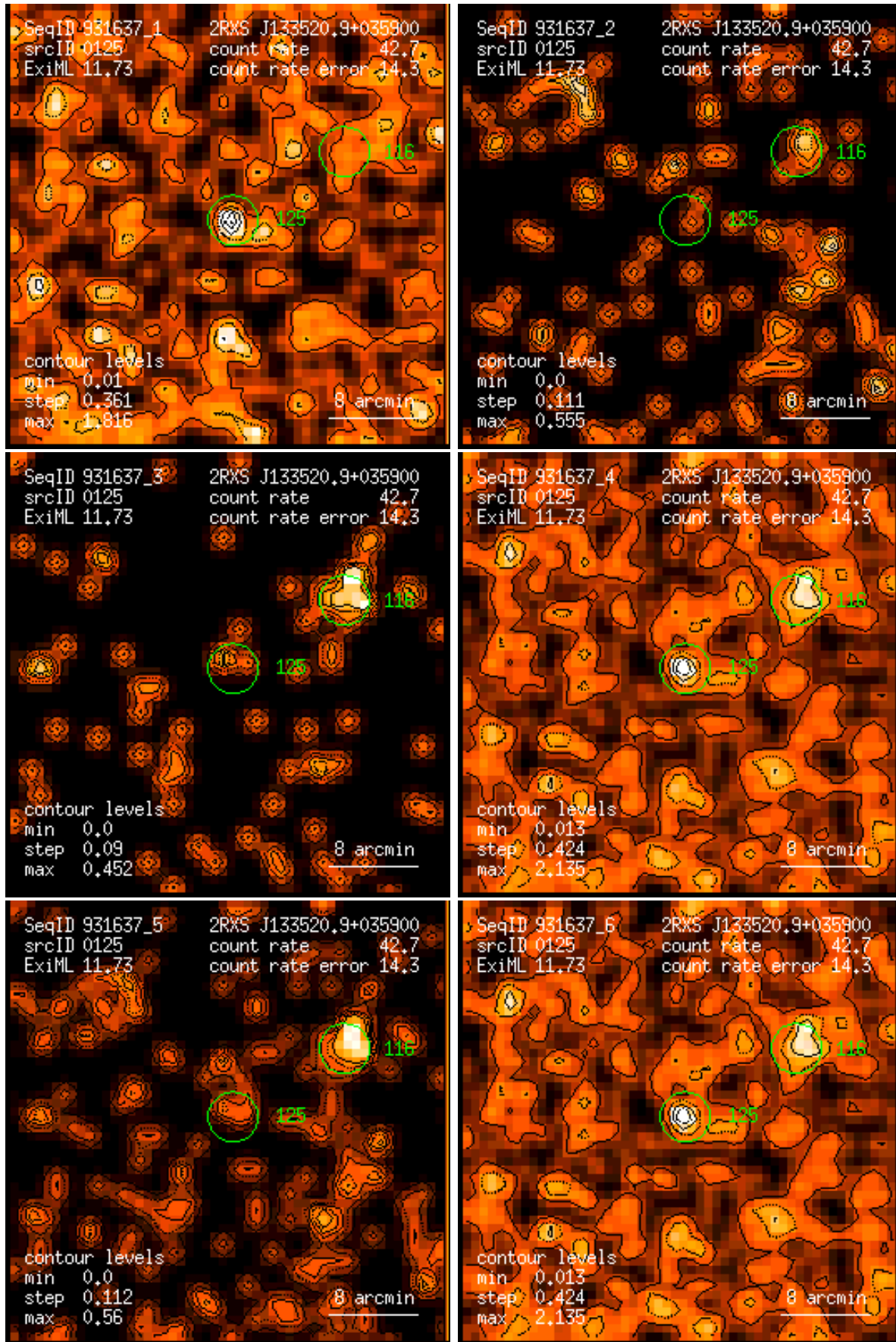
Figure 125: RASS 931637: detection 0125: band rate images, Gaussian filter: (1) PSPC channels 11 – 41, (2) 52 – 90, (3) 91 – 201, (4) 11 – 235, (5) 52 – 201, (6) 11 – 201. Broad band rates in counts/ks. Band rate contour levels in counts/ks/arcmin 2 .
