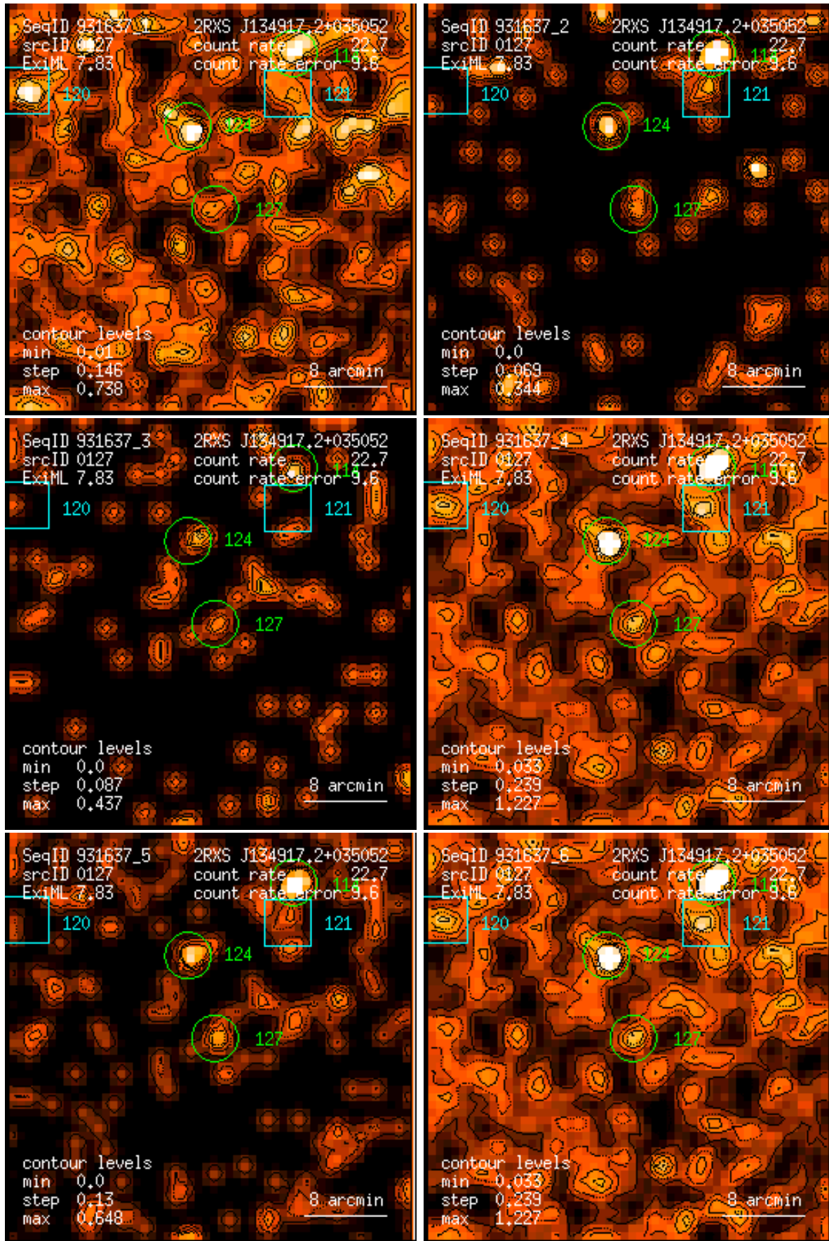
Figure 127: RASS 931637: detection 0127: band rate images, Gaussian filter: (1) PSPC channels 11 – 41, (2) 52 – 90, (3) 91 – 201, (4) 11 – 235, (5) 52 – 201, (6) 11 – 201. Broad band rates in counts/ks. Band rate contour levels in counts/ks/arcmin 2 .
