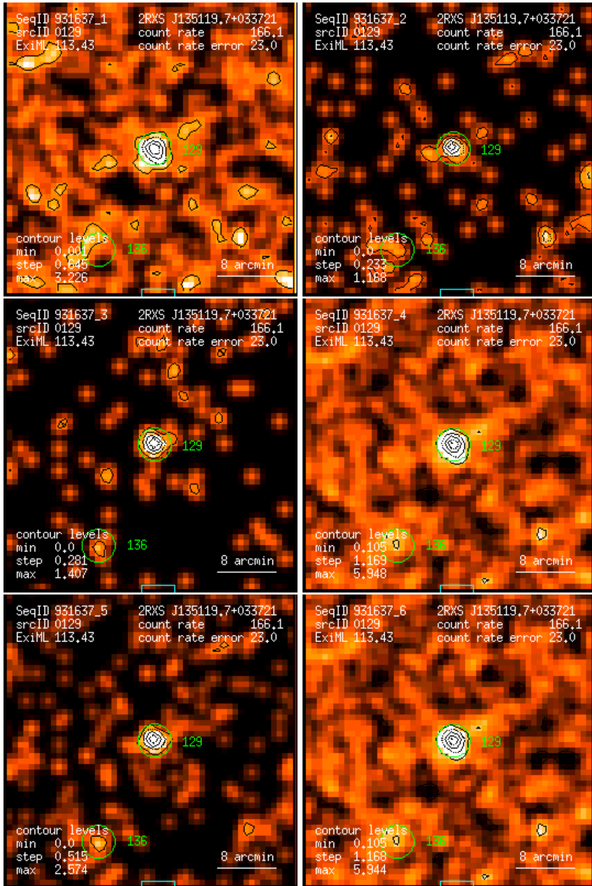
Figure 129: RASS 931637: detection 0129: band rate images, Gaussian filter: (1) PSPC channels 11 – 41, (2) 52 – 90, (3) 91 – 201, (4) 11 – 235, (5) 52 – 201, (6) 11 – 201. Broad band rates in counts/ks. Band rate contour levels in counts/ks/arcmin 2 .
