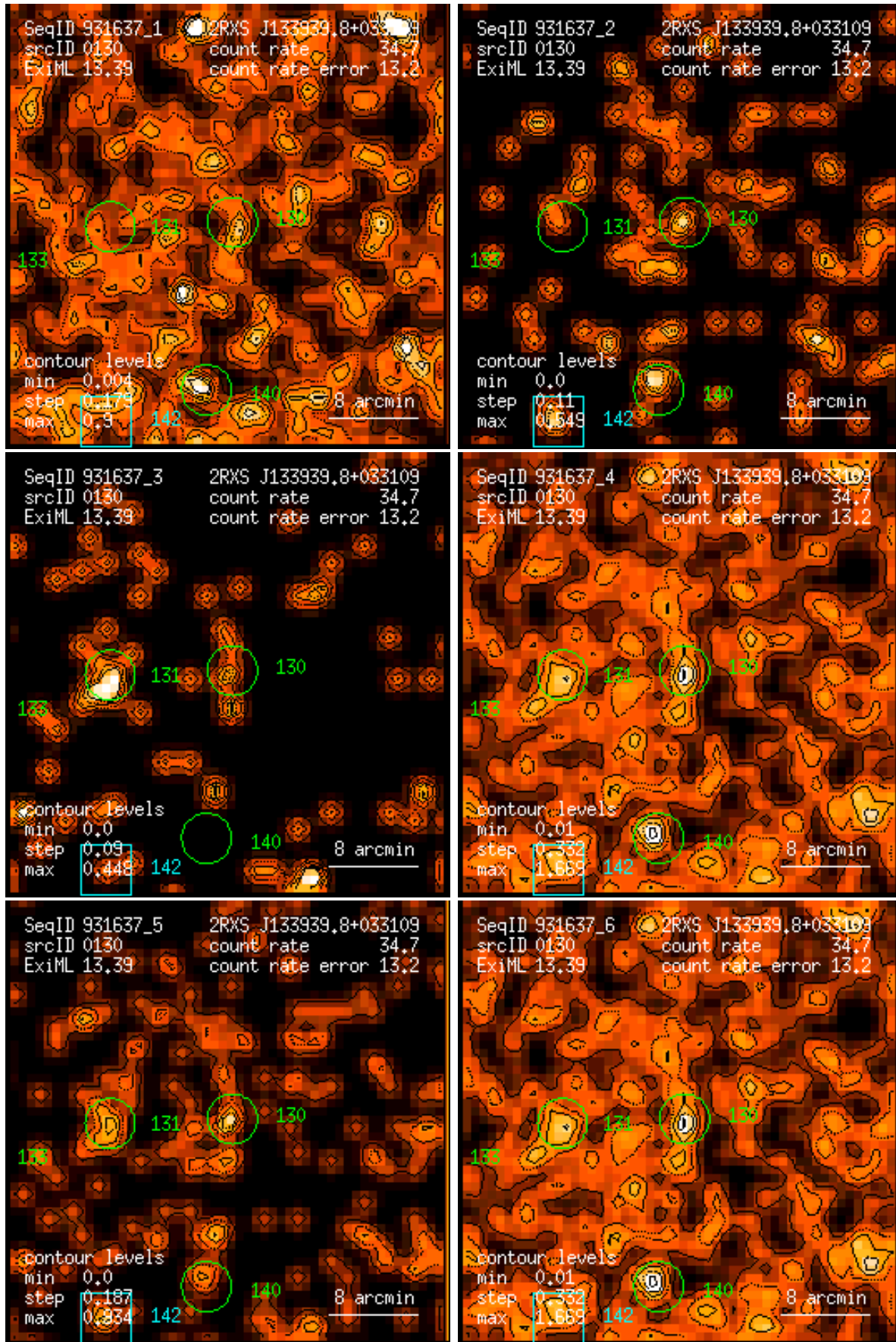
Figure 130: RASS 931637: detection 0130: band rate images, Gaussian filter: (1) PSPC channels 11 – 41, (2) 52 – 90, (3) 91 – 201, (4) 11 – 235, (5) 52 – 201, (6) 11 – 201. Broad band rates in counts/ks. Band rate contour levels in counts/ks/arcmin 2 .
