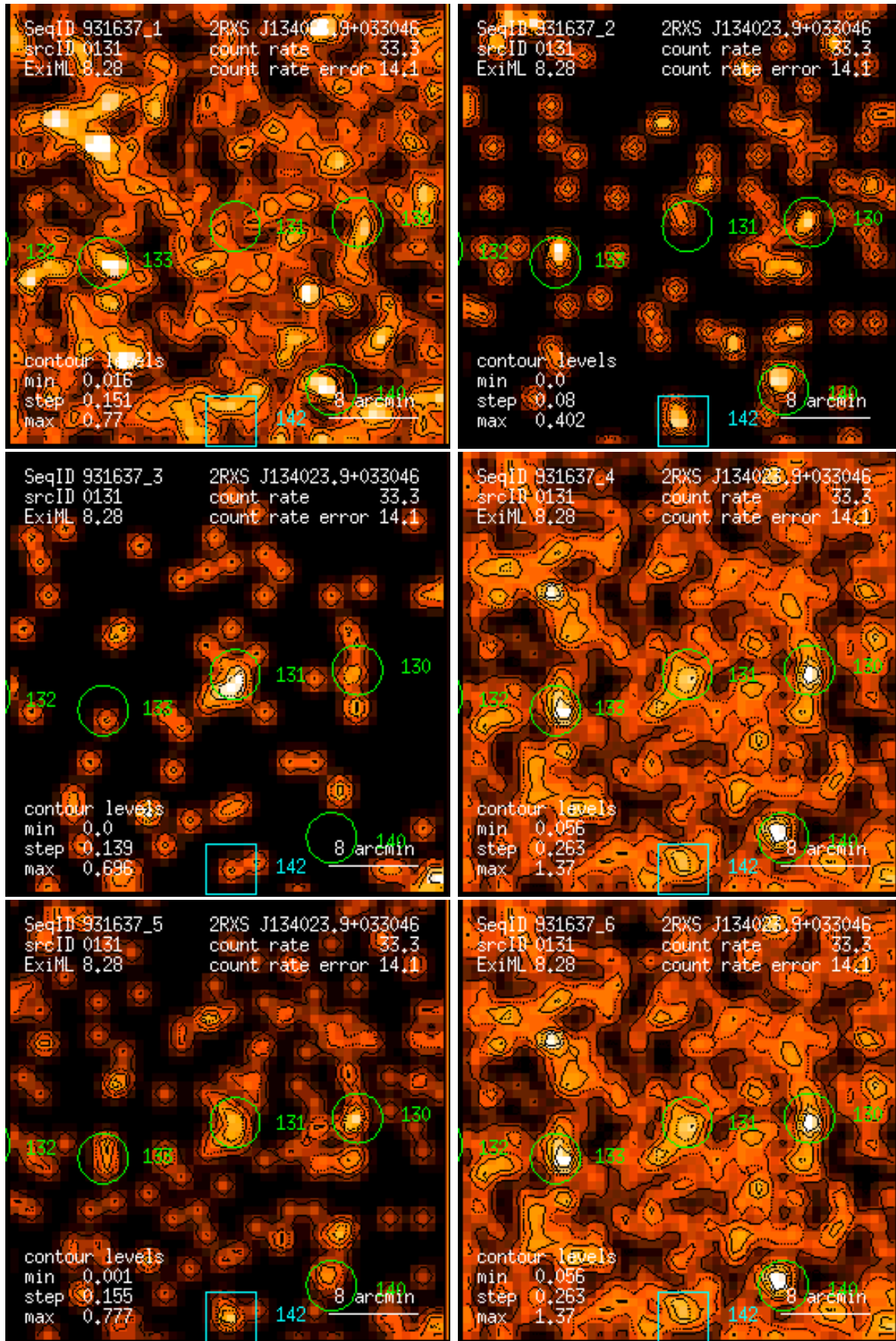
Figure 131: RASS 931637: detection 0131: band rate images, Gaussian filter: (1) PSPC channels 11 – 41, (2) 52 – 90, (3) 91 – 201, (4) 11 – 235, (5) 52 – 201, (6) 11 – 201. Broad band rates in counts/ks. Band rate contour levels in counts/ks/arcmin 2 .
