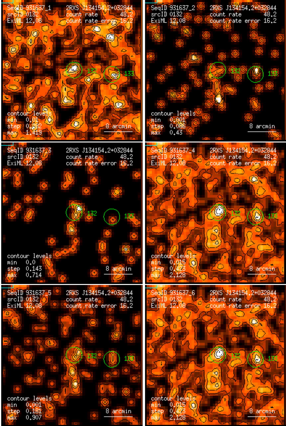
Figure 132: RASS 931637: detection 0132: band rate images, Gaussian filter: (1) PSPC channels 11 – 41, (2) 52 – 90, (3) 91 – 201, (4) 11 – 235, (5) 52 – 201, (6) 11 – 201. Broad band rates in counts/ks. Band rate contour levels in counts/ks/arcmin 2 .
