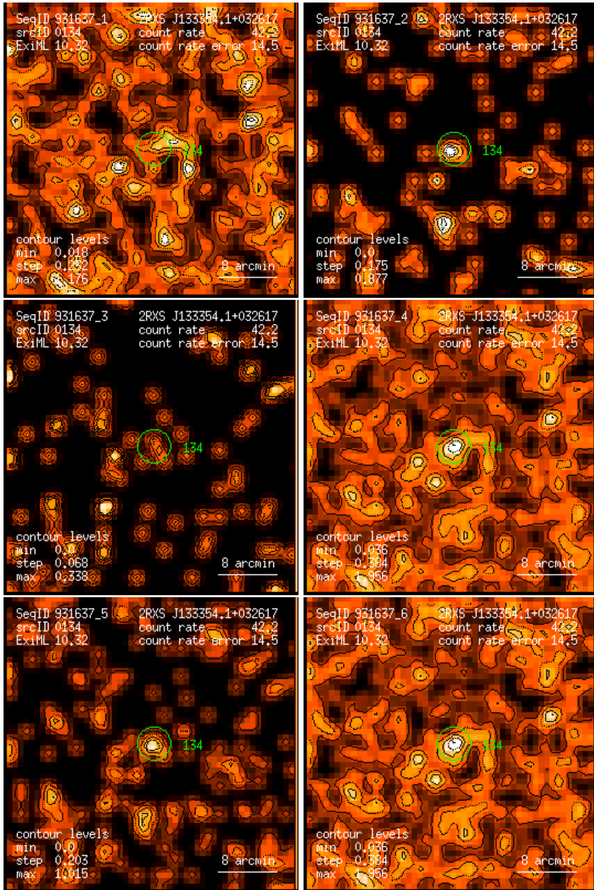
Figure 134: RASS 931637: detection 0134: band rate images, Gaussian filter: (1) PSPC channels 11 – 41, (2) 52 – 90, (3) 91 – 201, (4) 11 – 235, (5) 52 – 201, (6) 11 – 201. Broad band rates in counts/ks. Band rate contour levels in counts/ks/arcmin 2 .
