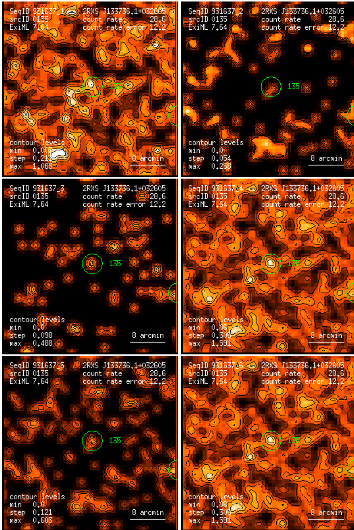
Figure 135: RASS 931637: detection 0135: band rate images, Gaussian filter: (1) PSPC channels 11 – 41, (2) 52 – 90, (3) 91 – 201, (4) 11 – 235, (5) 52 – 201, (6) 11 – 201. Broad band rates in counts/ks. Band rate contour levels in counts/ks/arcmin 2 .
