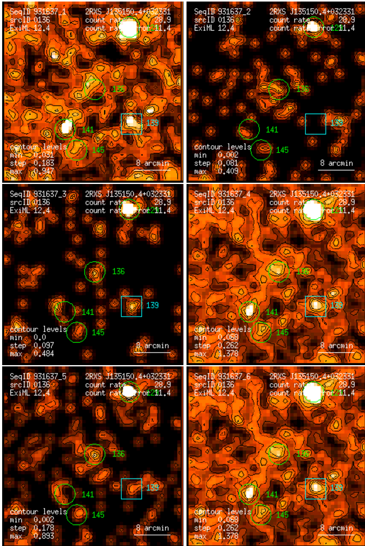
Figure 136: RASS 931637: detection 0136: band rate images, Gaussian filter: (1) PSPC channels 11 – 41, (2) 52 – 90, (3) 91 – 201, (4) 11 – 235, (5) 52 – 201, (6) 11 – 201. Broad band rates in counts/ks. Band rate contour levels in counts/ks/arcmin 2 .
