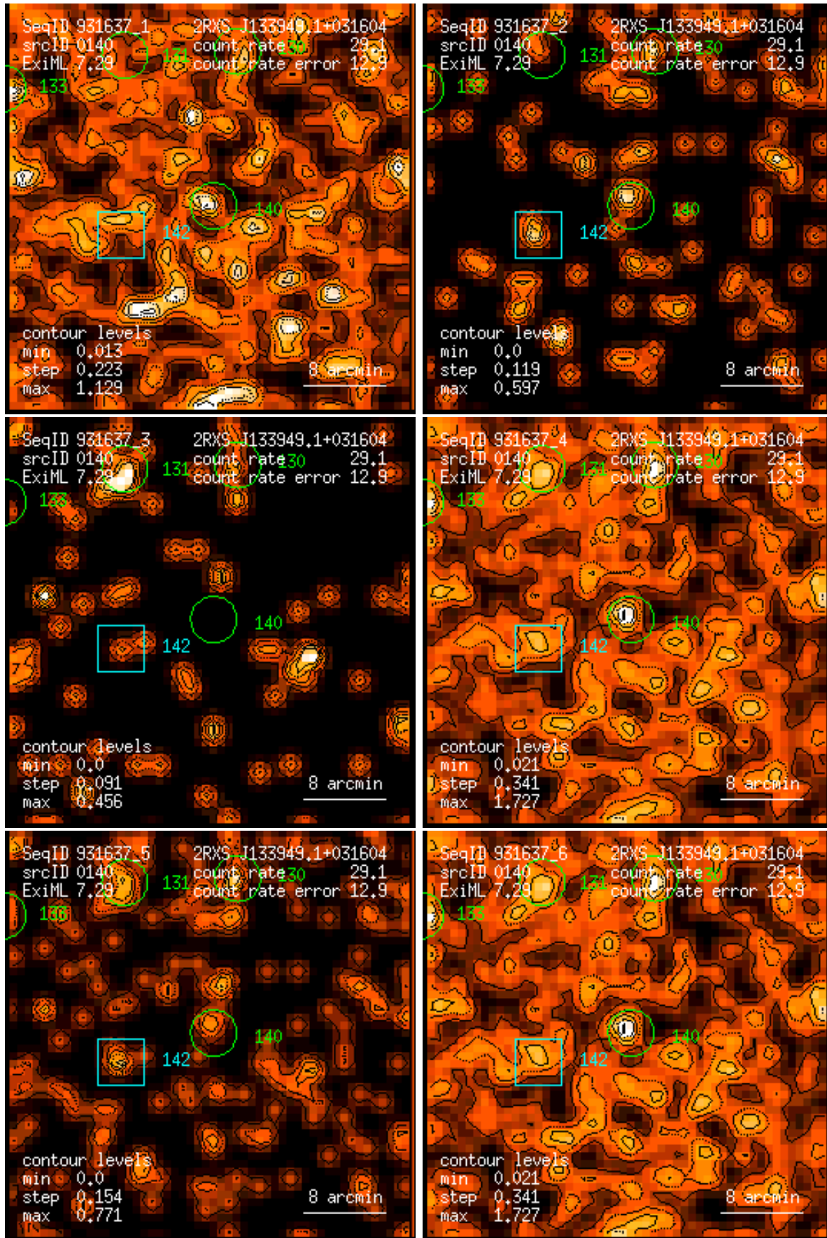
Figure 140: RASS 931637: detection 0140: band rate images, Gaussian filter: (1) PSPC channels 11 – 41, (2) 52 – 90, (3) 91 – 201, (4) 11 – 235, (5) 52 – 201, (6) 11 – 201. Broad band rates in counts/ks. Band rate contour levels in counts/ks/arcmin 2 .
