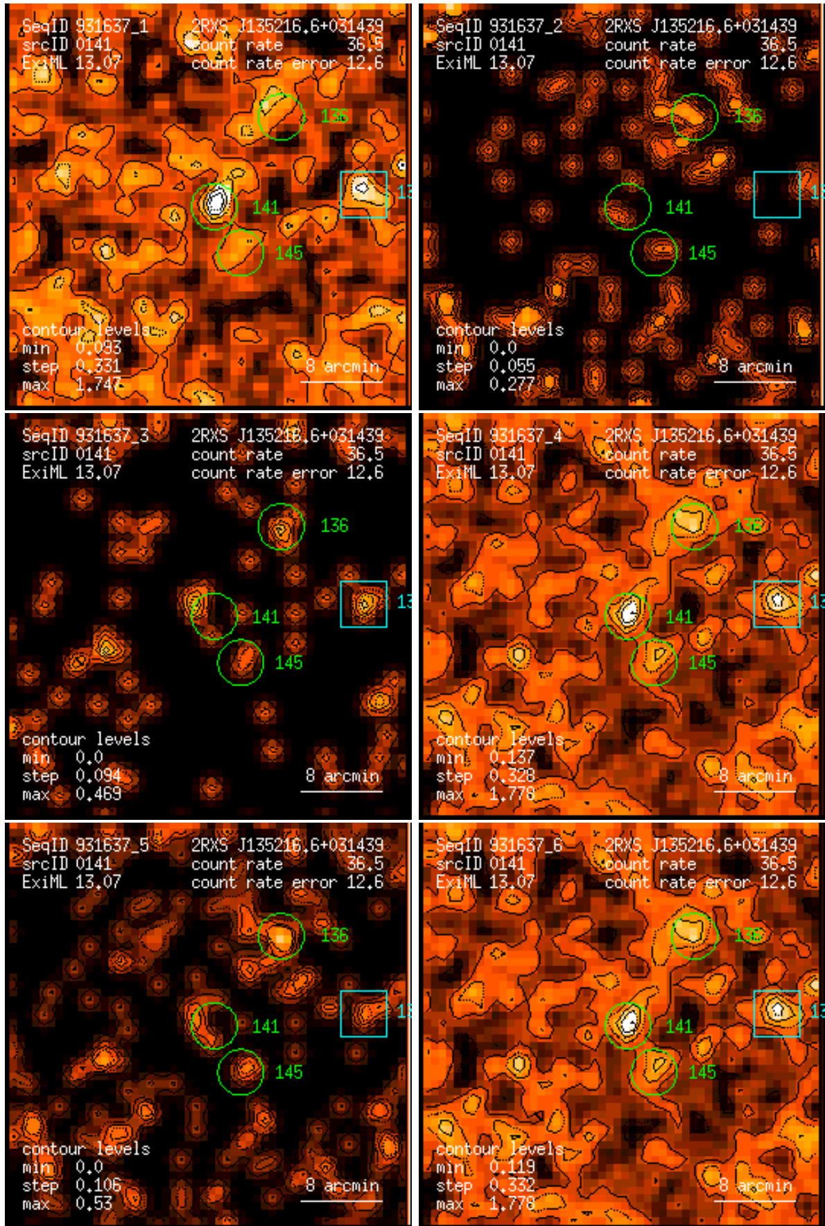
Figure 141: RASS 931637: detection 0141: band rate images, Gaussian filter: (1) PSPC channels 11 – 41, (2) 52 – 90, (3) 91 – 201, (4) 11 – 235, (5) 52 – 201, (6) 11 – 201. Broad band rates in counts/ks. Band rate contour levels in counts/ks/arcmin 2 .
