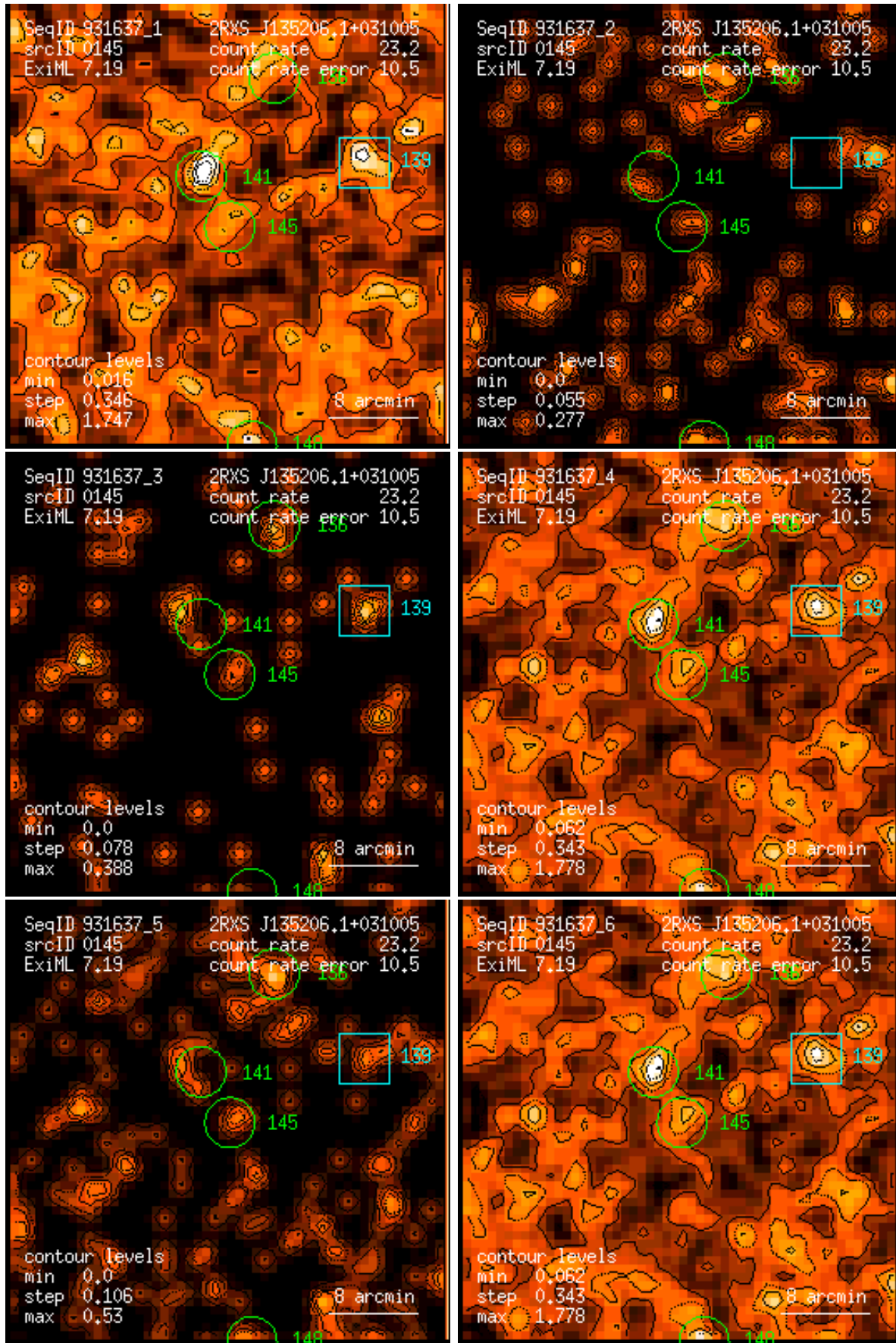
Figure 145: RASS 931637: detection 0145: band rate images, Gaussian filter: (1) PSPC channels 11 – 41, (2) 52 – 90, (3) 91 – 201, (4) 11 – 235, (5) 52 – 201, (6) 11 – 201. Broad band rates in counts/ks. Band rate contour levels in counts/ks/arcmin 2 .
