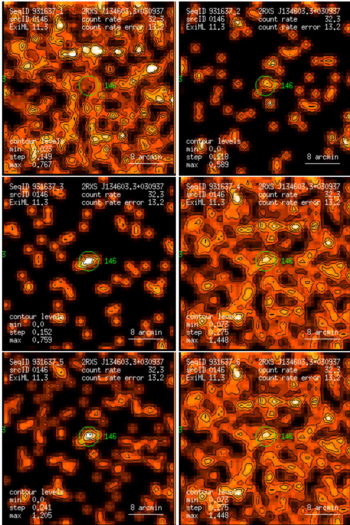
Figure 146: RASS 931637: detection 0146: band rate images, Gaussian filter: (1) PSPC channels 11 – 41, (2) 52 – 90, (3) 91 – 201, (4) 11 – 235, (5) 52 – 201, (6) 11 – 201. Broad band rates in counts/ks. Band rate contour levels in counts/ks/arcmin 2 .
