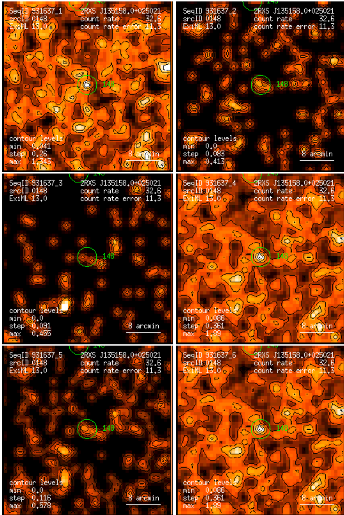
Figure 148: RASS 931637: detection 0148: band rate images, Gaussian filter: (1) PSPC channels 11 – 41, (2) 52 – 90, (3) 91 – 201, (4) 11 – 235, (5) 52 – 201, (6) 11 – 201. Broad band rates in counts/ks. Band rate contour levels in counts/ks/arcmin 2 .
