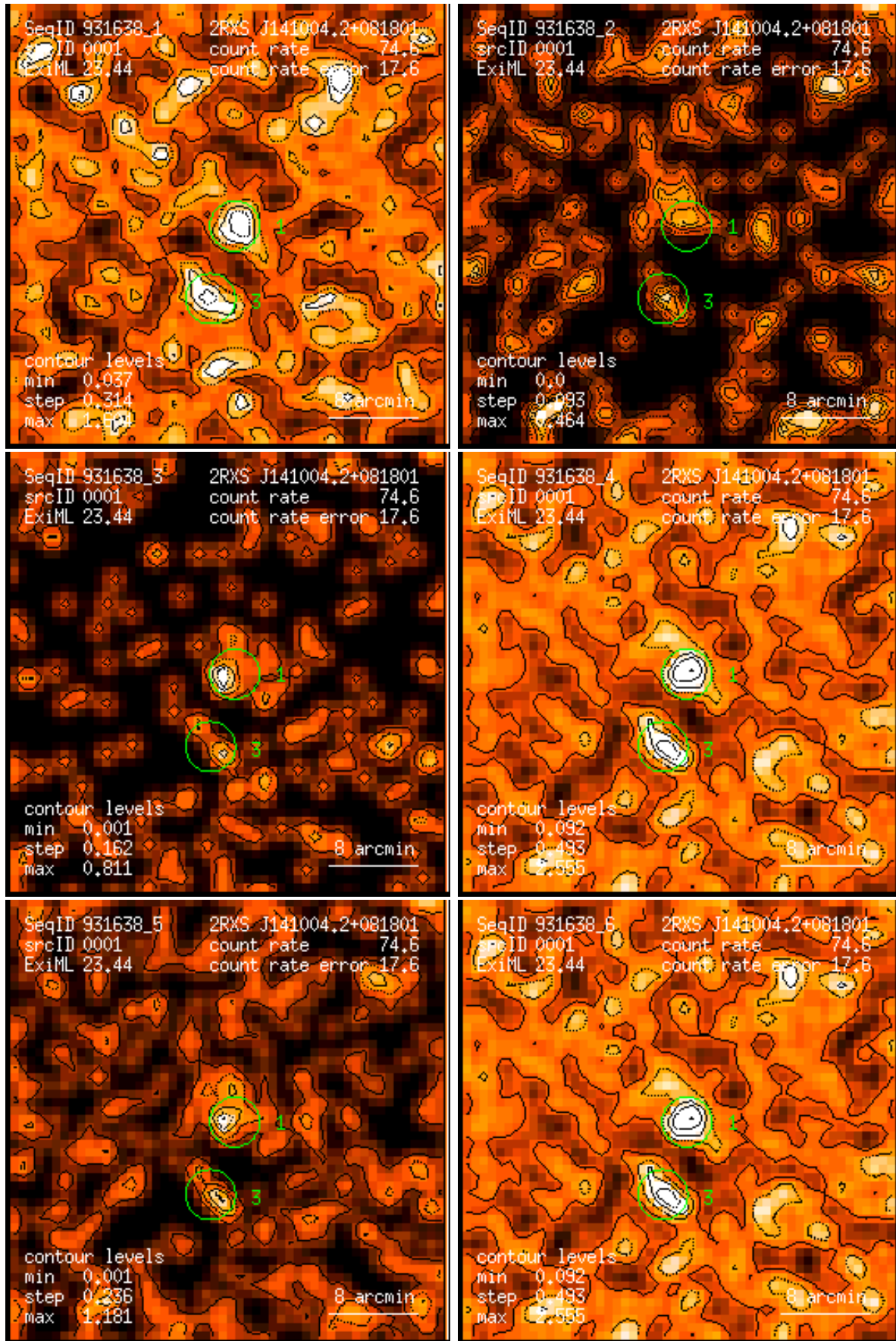
Figure 1: RASS 931638: detection 0001: band rate images, Gaussian filter: (1) PSPC channels 11 – 41, (2) 52 – 90, (3) 91 – 201, (4) 11 – 235, (5) 52 – 201, (6) 11 – 201. Broad band rates in counts/ks. Band rate contour levels in counts/ks/arcmin 2 .
