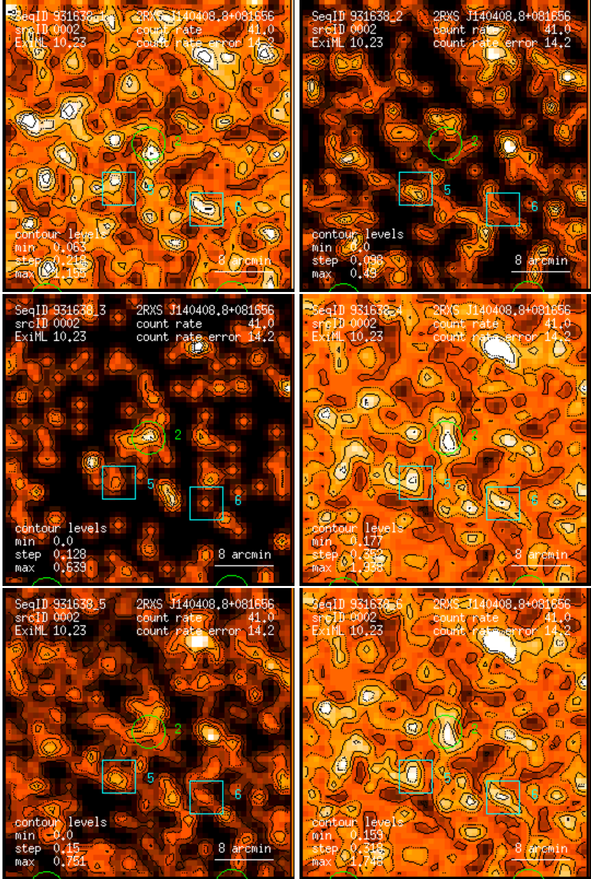
Figure 2: RASS 931638: detection 0002: band rate images, Gaussian filter: (1) PSPC channels 11 – 41, (2) 52 – 90, (3) 91 – 201, (4) 11 – 235, (5) 52 – 201, (6) 11 – 201. Broad band rates in counts/ks. Band rate contour levels in counts/ks/arcmin 2 .
