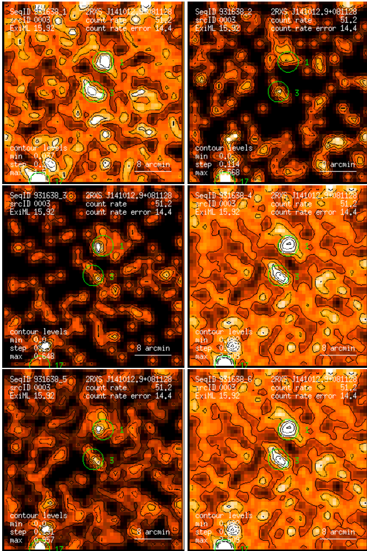
Figure 3: RASS 931638: detection 0003: band rate images, Gaussian filter: (1) PSPC channels 11 – 41, (2) 52 – 90, (3) 91 – 201, (4) 11 – 235, (5) 52 – 201, (6) 11 – 201. Broad band rates in counts/ks. Band rate contour levels in counts/ks/arcmin 2 .
