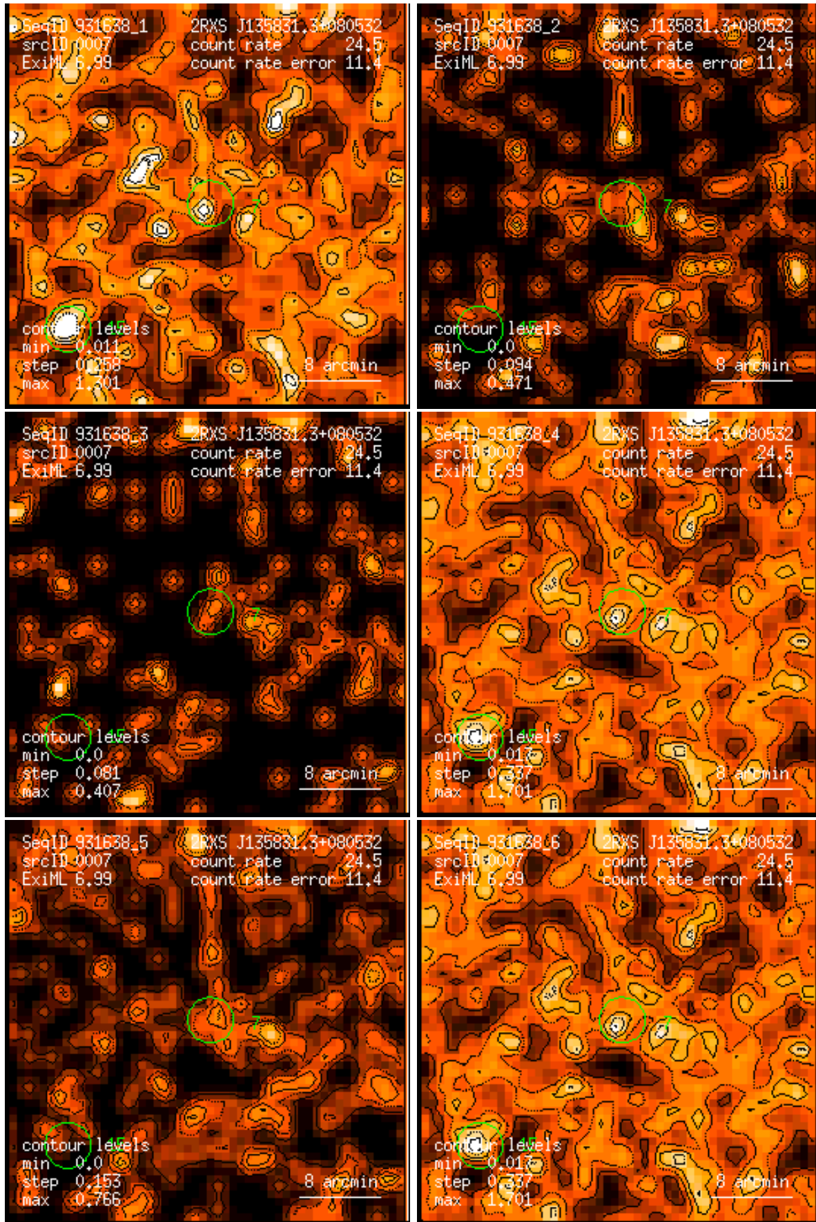
Figure 7: RASS 931638: detection 0007: band rate images, Gaussian filter: (1) PSPC channels 11 – 41, (2) 52 – 90, (3) 91 – 201, (4) 11 – 235, (5) 52 – 201, (6) 11 – 201. Broad band rates in counts/ks. Band rate contour levels in counts/ks/arcmin 2 .
