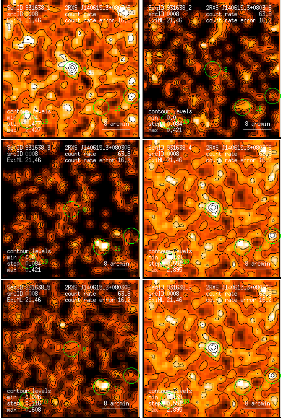
Figure 8: RASS 931638: detection 0008: band rate images, Gaussian filter: (1) PSPC channels 11 – 41, (2) 52 – 90, (3) 91 – 201, (4) 11 – 235, (5) 52 – 201, (6) 11 – 201. Broad band rates in counts/ks. Band rate contour levels in counts/ks/arcmin 2 .
