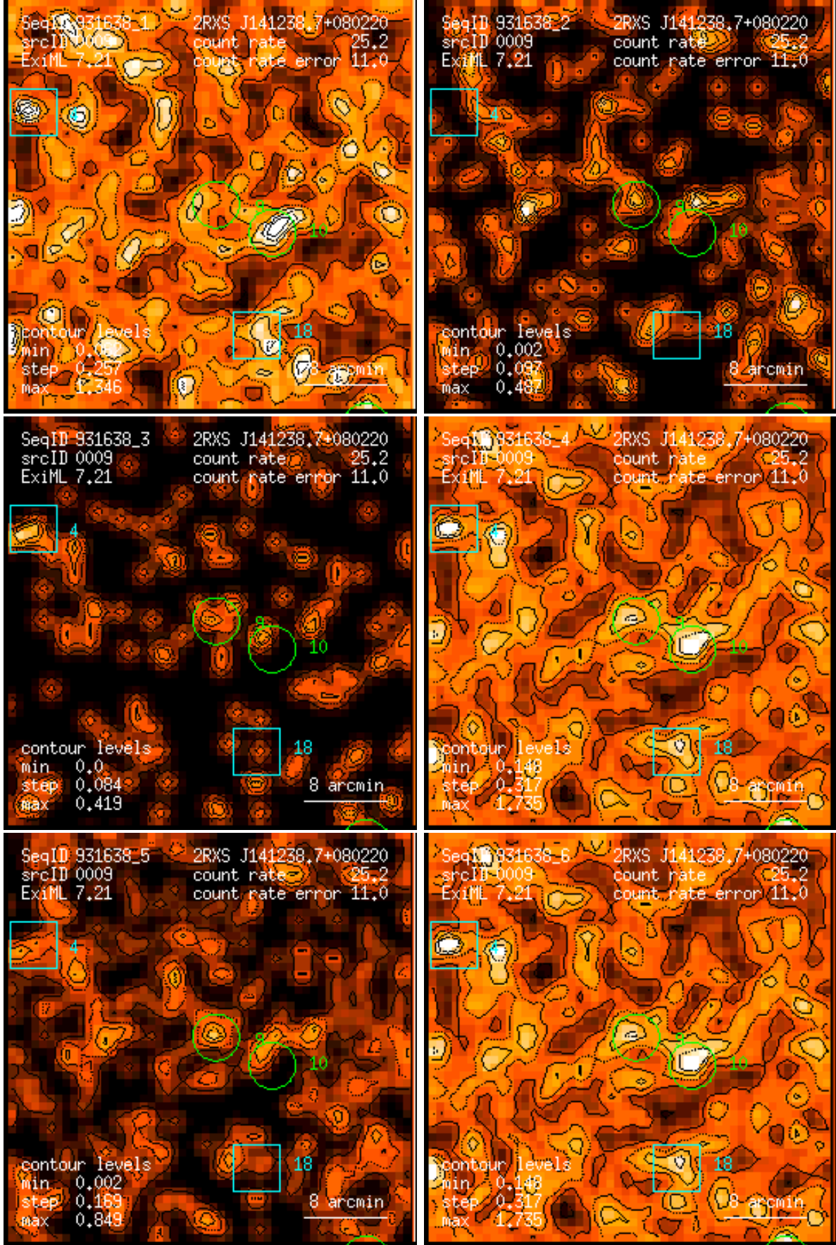
Figure 9: RASS 931638: detection 0009: band rate images, Gaussian filter: (1) PSPC channels 11 – 41, (2) 52 – 90, (3) 91 – 201, (4) 11 – 235, (5) 52 – 201, (6) 11 – 201. Broad band rates in counts/ks. Band rate contour levels in counts/ks/arcmin 2 .
