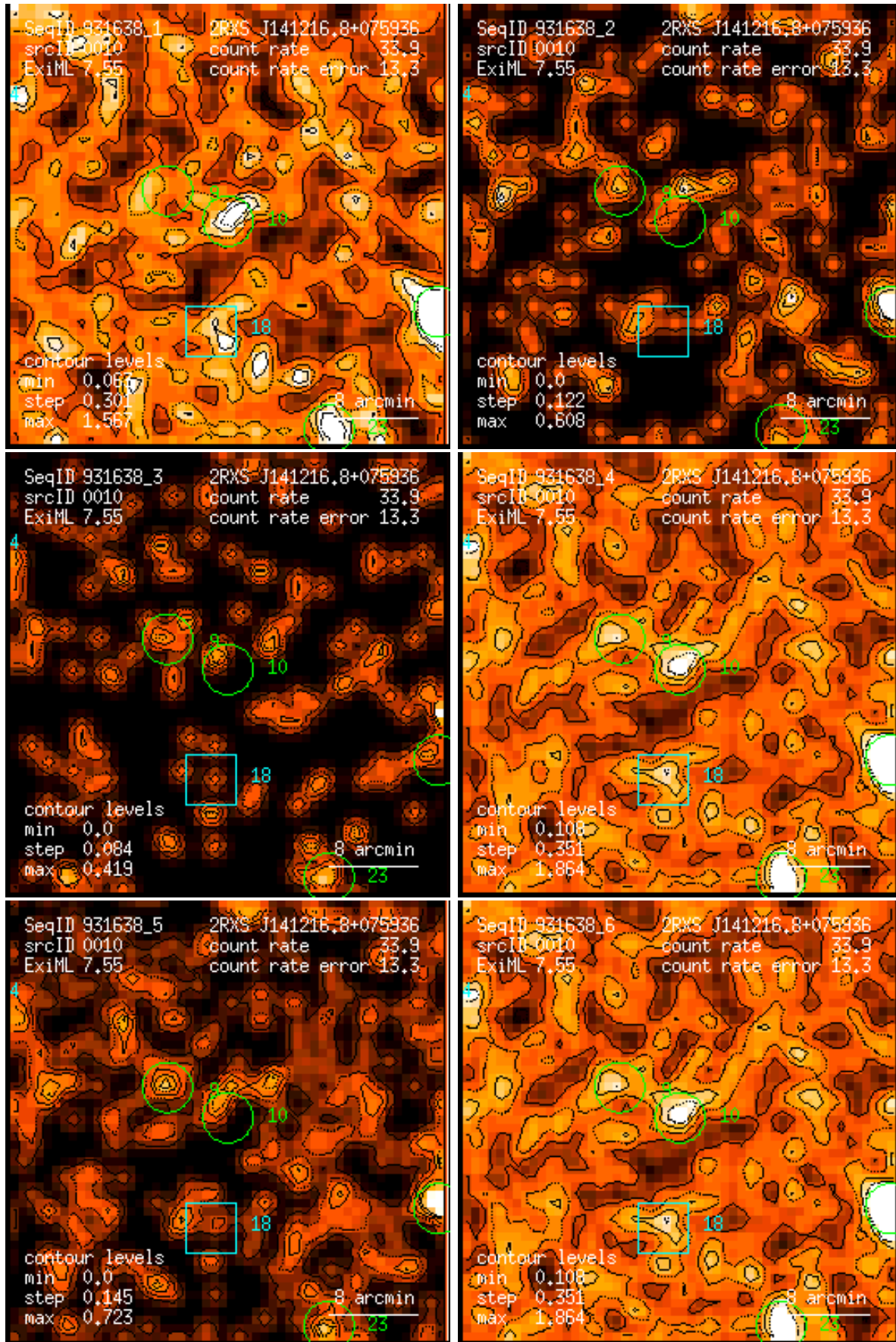
Figure 10: RASS 931638: detection 0010: band rate images, Gaussian filter: (1) PSPC channels 11 – 41, (2) 52 – 90, (3) 91 – 201, (4) 11 – 235, (5) 52 – 201, (6) 11 – 201. Broad band rates in counts/ks. Band rate contour levels in counts/ks/arcmin 2 .
