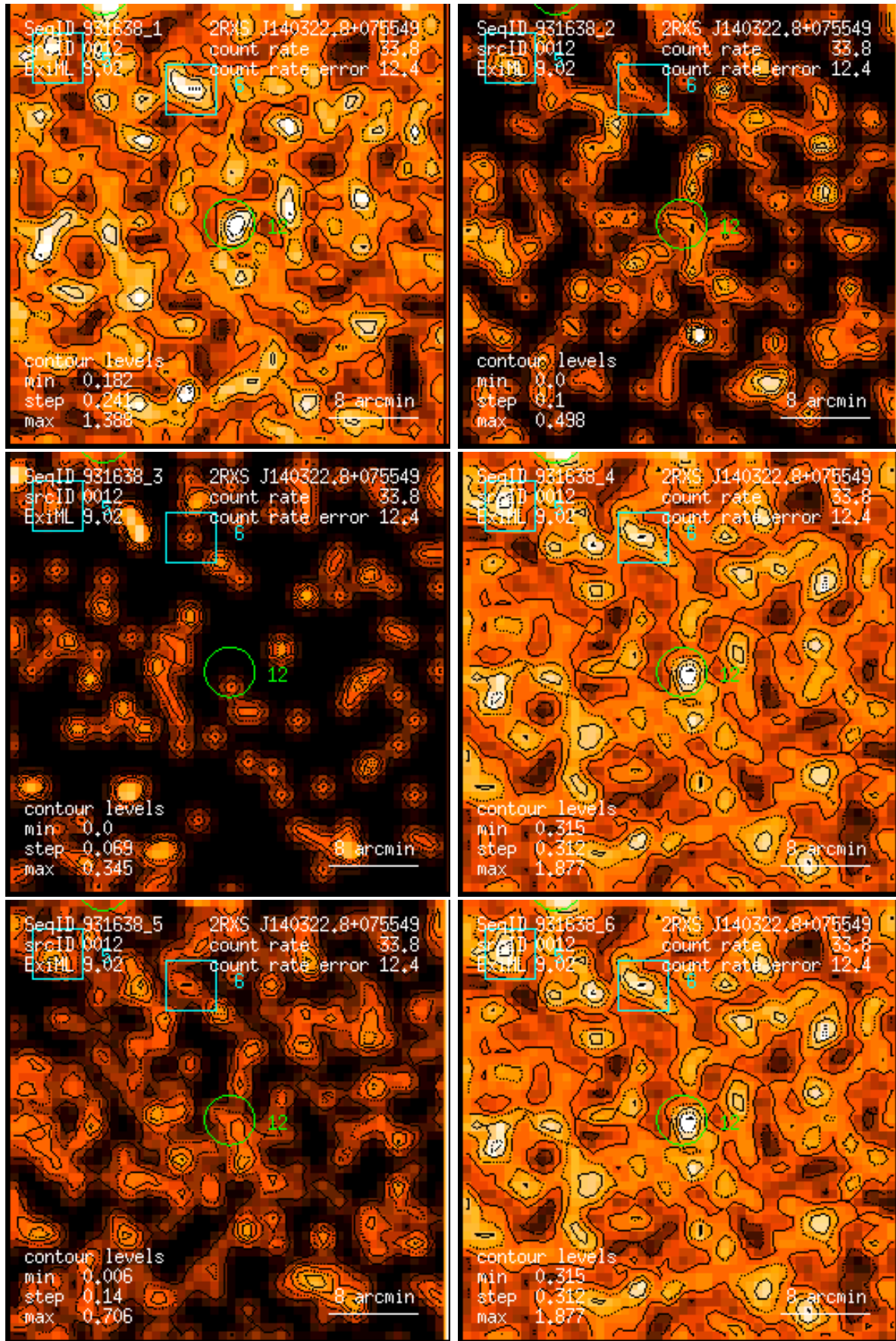
Figure 12: RASS 931638: detection 0012: band rate images, Gaussian filter: (1) PSPC channels 11 – 41, (2) 52 – 90, (3) 91 – 201, (4) 11 – 235, (5) 52 – 201, (6) 11 – 201. Broad band rates in counts/ks. Band rate contour levels in counts/ks/arcmin 2 .
